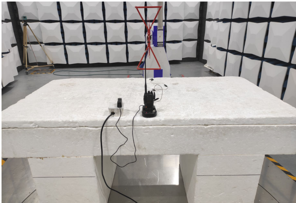
Radiated Emissions Rear View (Below 1GHz)
