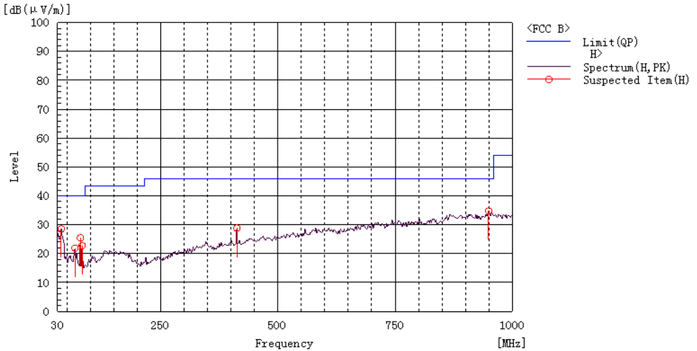
Radiated Emission Test –Horizontal -3m Below 1G
