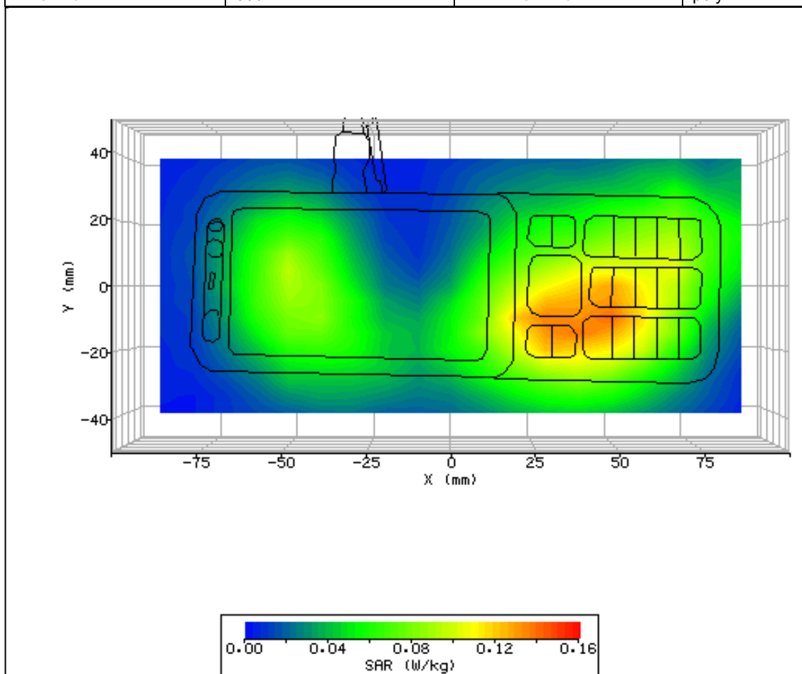
Figure 12: SAR Body Testing Results for the SS11-J01 Mobile Handset at 1880MHz.
