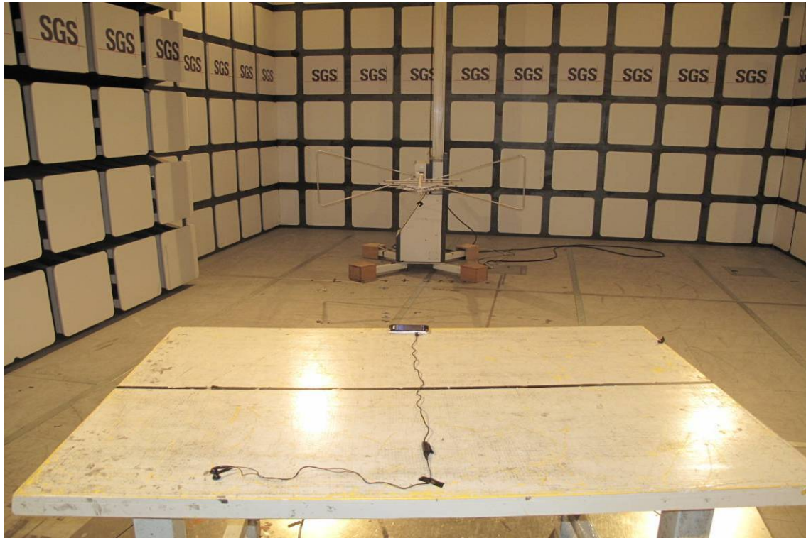
Radiated Emission Test Setup Photo (config 2)
