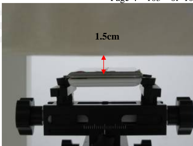
Fig.11 Body worn- EUT front to flat phantom and distance between flat phantom and mobile phone is 1.5 cm
