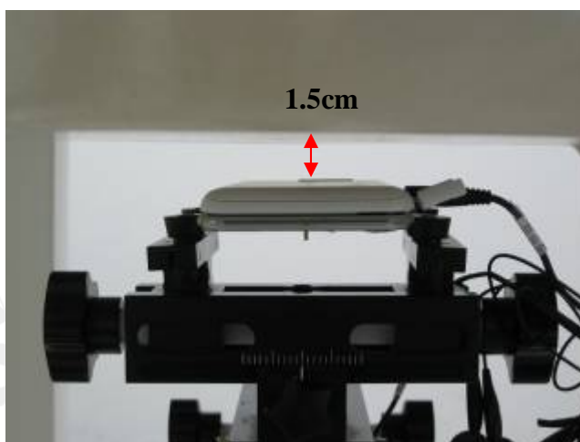
Fig.13 Body worn- EUT back to flat phantom and distance between flat phantom and mobile phone is 1.5 cm with headset.
