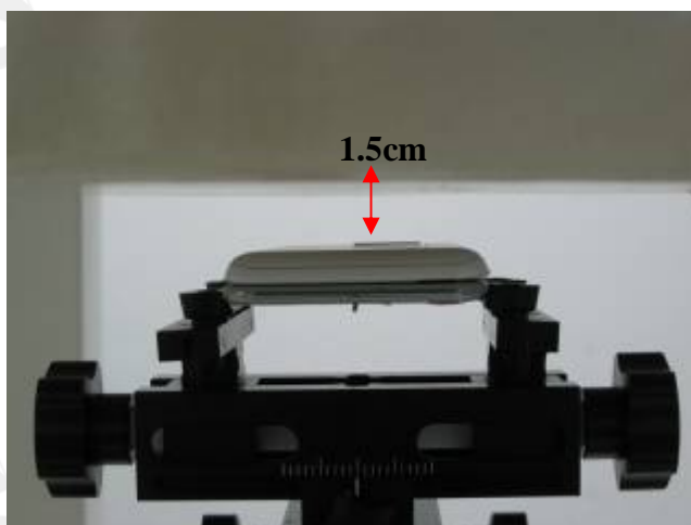
Fig.12 Body worn- EUT back to flat phantom and distance between flat phantom and mobile phone is 1.5 cm
