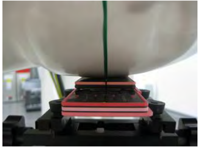
Fig.9 Left Head Section / Cheek-Touch Position_ Slider open
