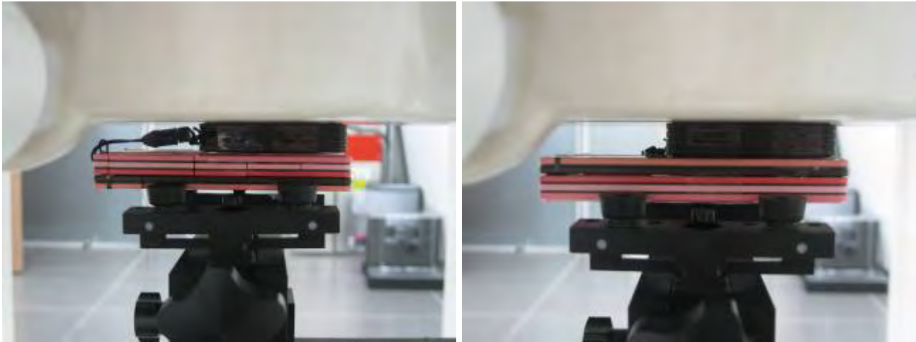
Fig.18 Body worn- EUT back or front to flat phantom and repeated with earphone cable case(position 1 & 2)
