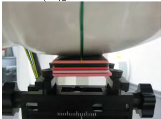
Fig.5 Left Head Section / Cheek-Touch Position_ Slider close
