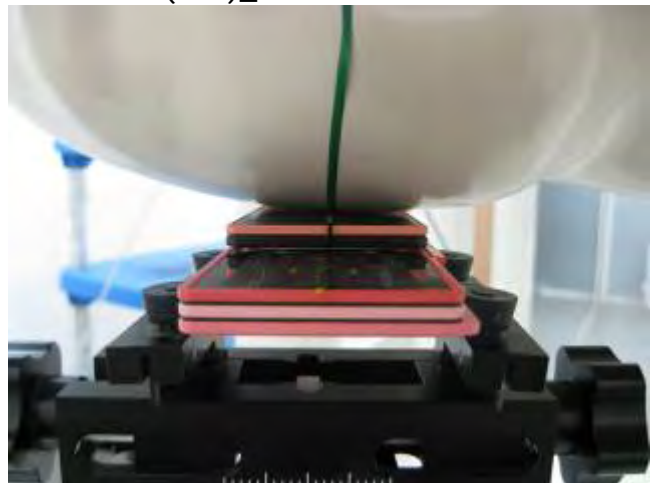
Fig.7 Right Head Section / Cheek-Touch Position_ Slider open
