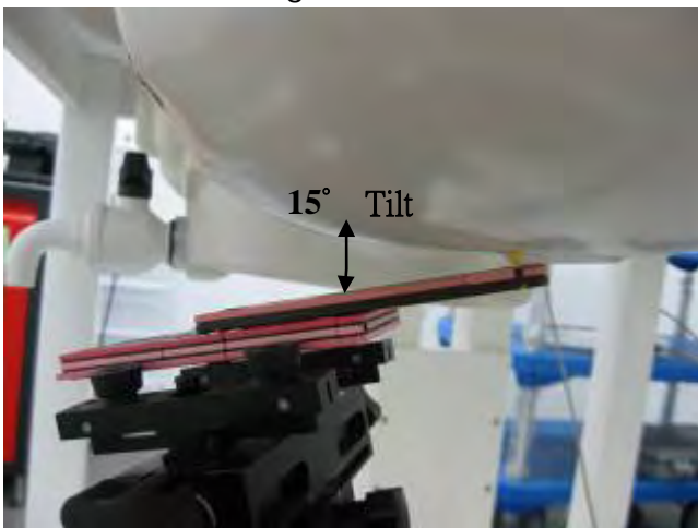
Fig.10 Left Head Section / Ear-Tilt Position(15°)_ Slider open
