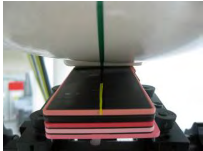
Fig.6 Left Head Section / Ear-Tilt Position(15°)_ Slider close
