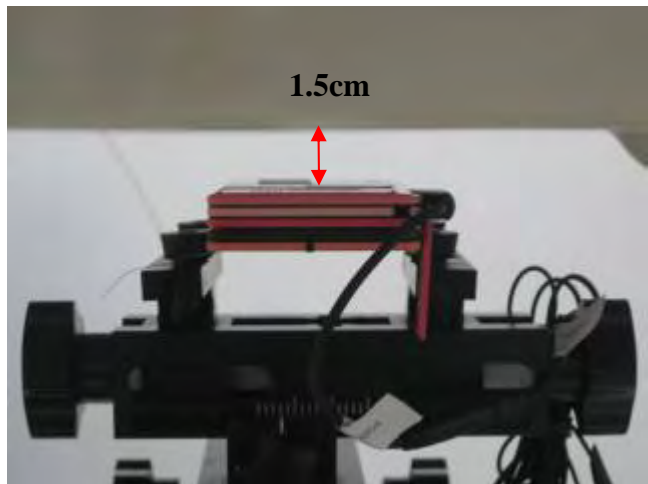
Fig.13 Body worn- EUT back to flat phantom and distance between flat phantom and mobile phone is 1.5 cm with headset
