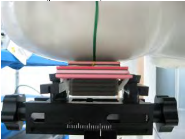
Fig.16 Right Head Section / Cheek-Touch Position_ Slider open repeated with earphone cable case(position 1 & 2)
