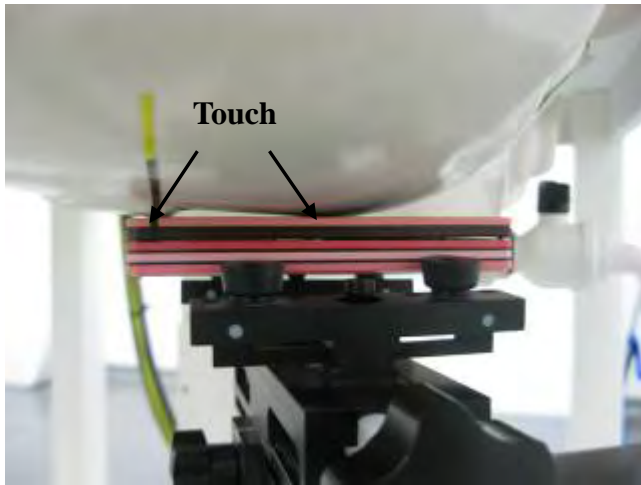
Fig.3 Right Head Section / Cheek-Touch Position_ Slider close
