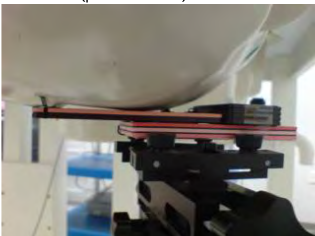
Fig.17 Right Head Section / Cheek-Touch Position_ Slider open repeated with earphone cable case(position 3 & 4)
