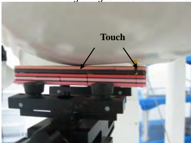
Fig.5 Left Head Section / Cheek-Touch Position_ Slider close
