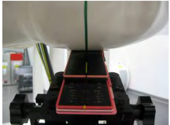
Fig.10 Left Head Section / Ear-Tilt Position(15°)_ Slider open
