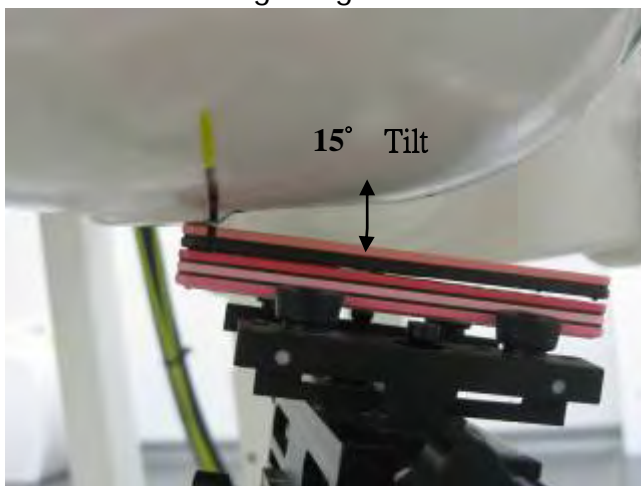
Fig.4 Right Head Section / Ear-Tilt Position(15°)_ Slider close
