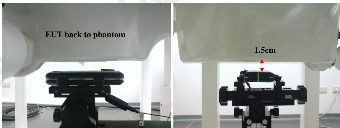
Fig.13 Body worn- EUT back to flat phantom and distance between flat phantom and mobile phone is 1.5 cm with headset
