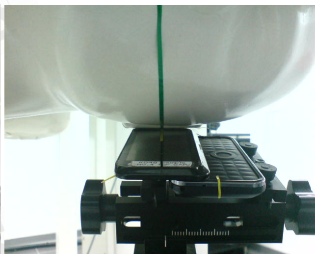
Fig.10 Left Head Section / Ear-Tilt Position(15°)_ Slider on
