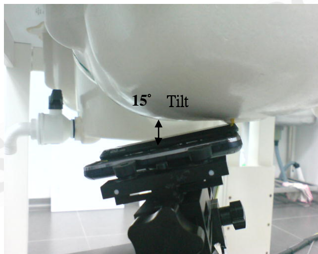
Fig.10 Left Head Section / Ear-Tilt Position(15°)_ Slider on
