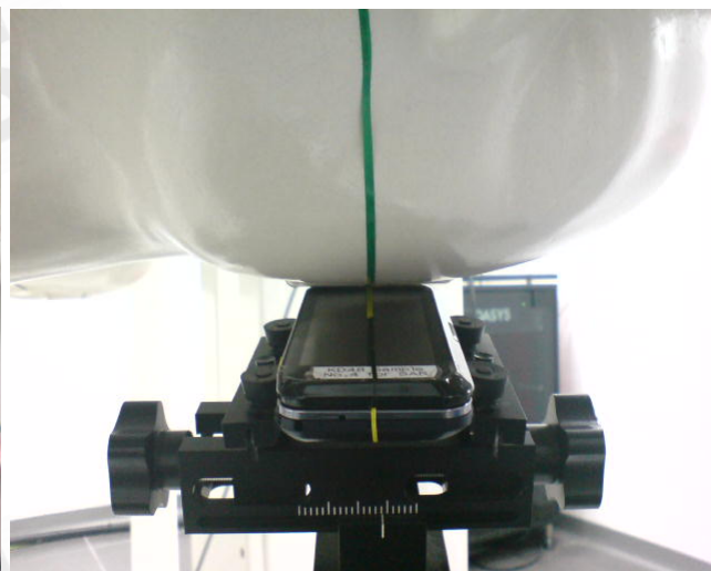
Fig.6 Left Head Section / Ear-Tilt Position(15°)_ Slider off
