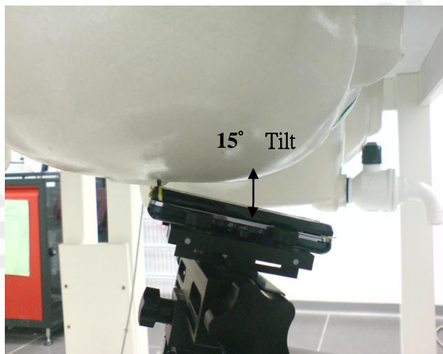
Fig.4 Right Head Section / Ear-Tilt Position(15°)_ Slider off
