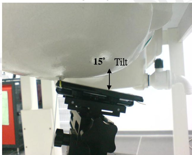
Fig.8 Right Head Section / Ear-Tilt Position(15°)_ Slider on
