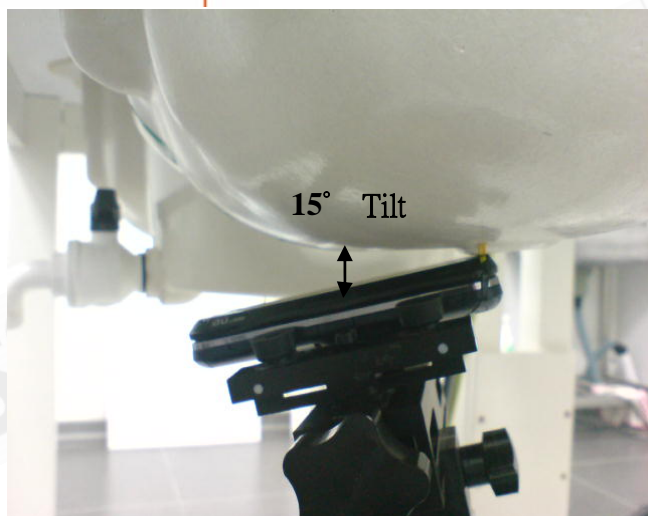
Fig.6 Left Head Section / Ear-Tilt Position(15°)_ Slider off
