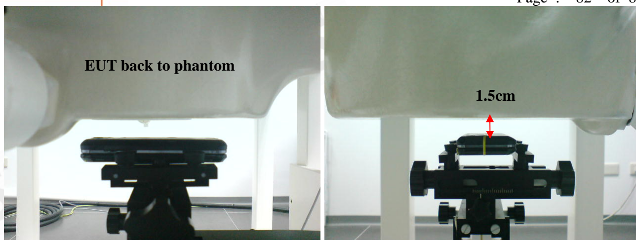
Fig.12 Body worn- EUT back to flat phantom and distance between flat phantom and mobile phone is 1.5 cm
