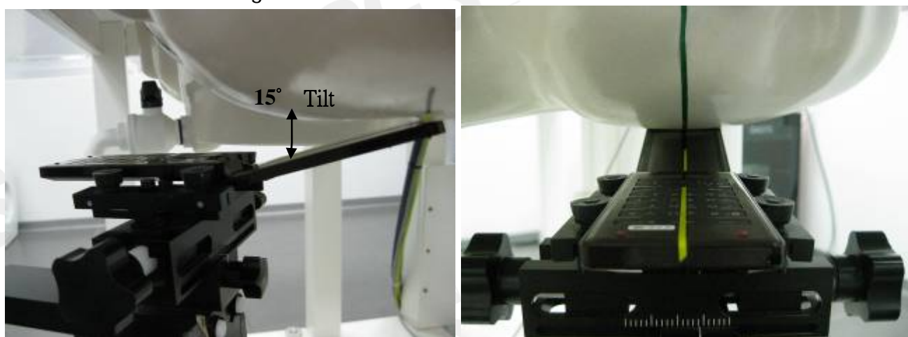
Fig.6 Left Head Section / Ear-Tilt Position(15°)
