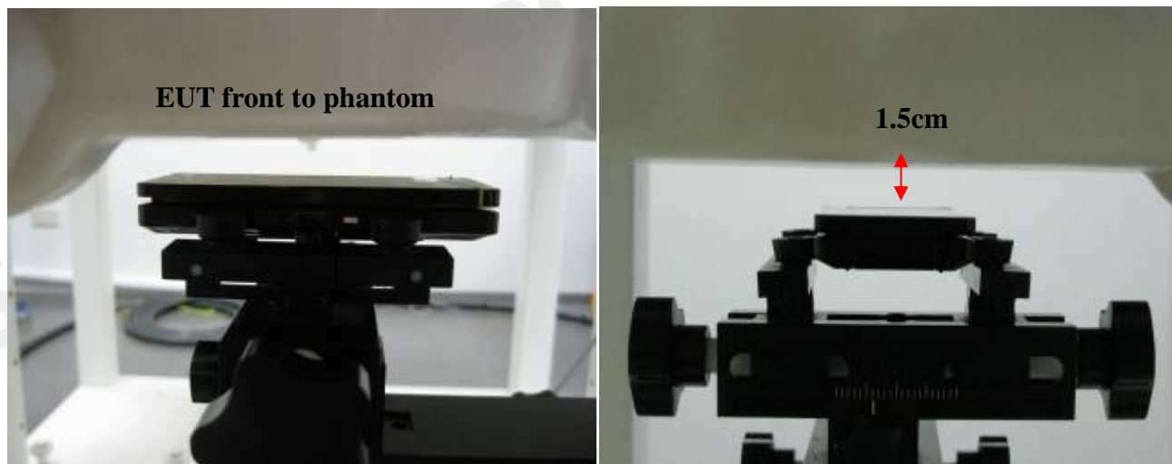
Fig.8 Body worn- EUT back to flat phantom and distance between flat phantom and mobile phone is 1.5 cm
