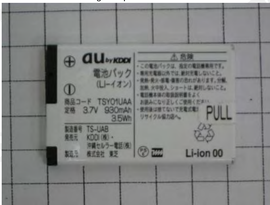
Fig.12 Front view of Battery
