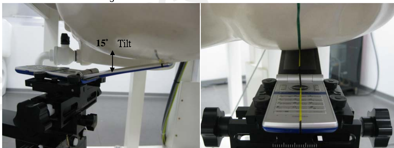
Fig.6 Left Head Section / Ear-Tilt Position(15°)
