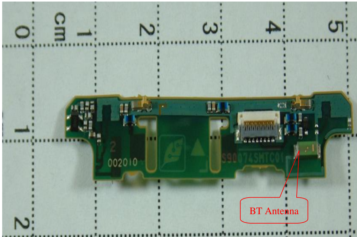
Sub PCB (Front)
