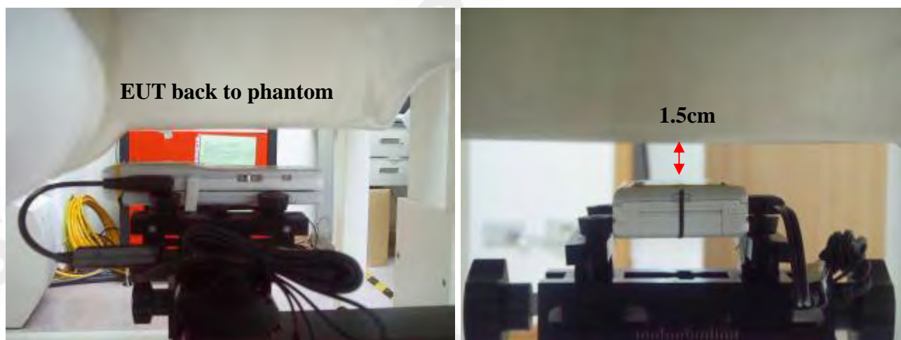
Fig.9 Body worn- EUT back to flat phantom with headset and distance between flat phantom and mobile phone is 1.5 cm
