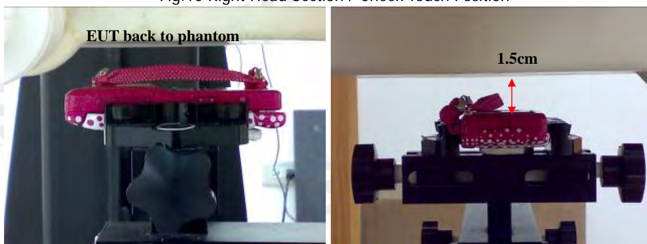
Fig.11 Body worn- EUT back to flat phantom and distance between flat phantom and mobile phone is 1.5 cm
