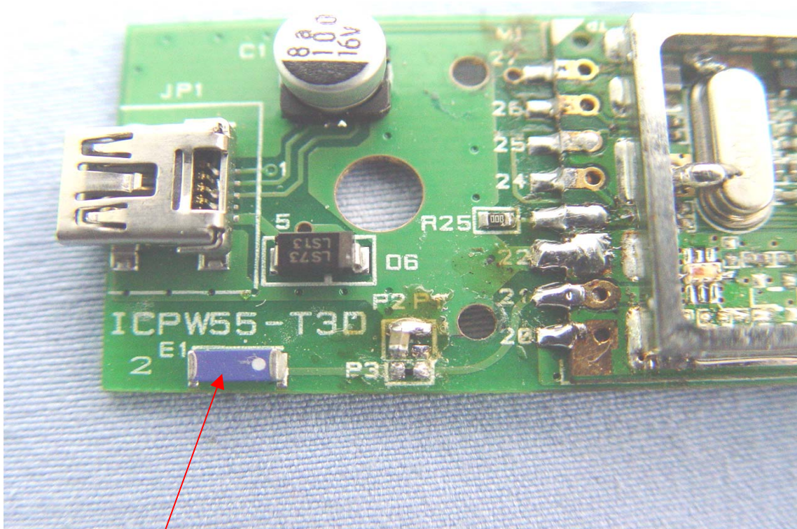
Chip Antenna
