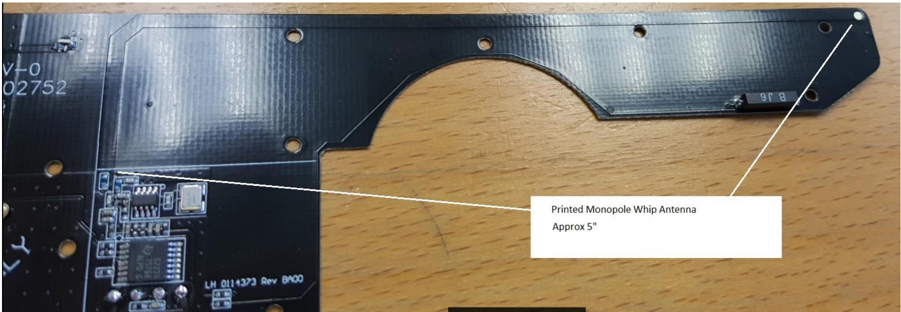
Verilock RbA CSMT PCB – Showing Antenna
