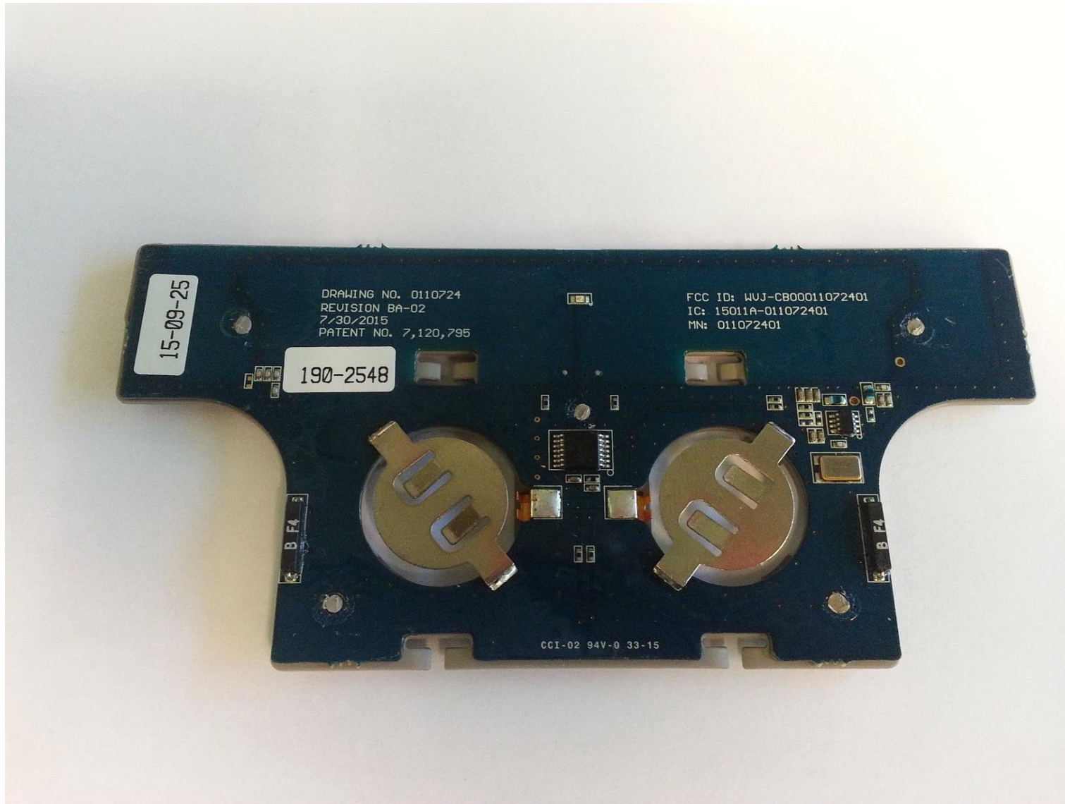
Hinge Door Photo – Assembly in Plastic Carrier - FRONT
