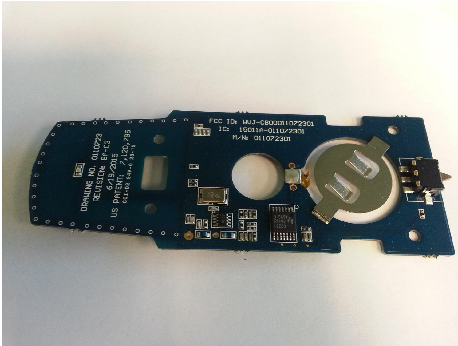
Gliding Door – PCB FRONT
