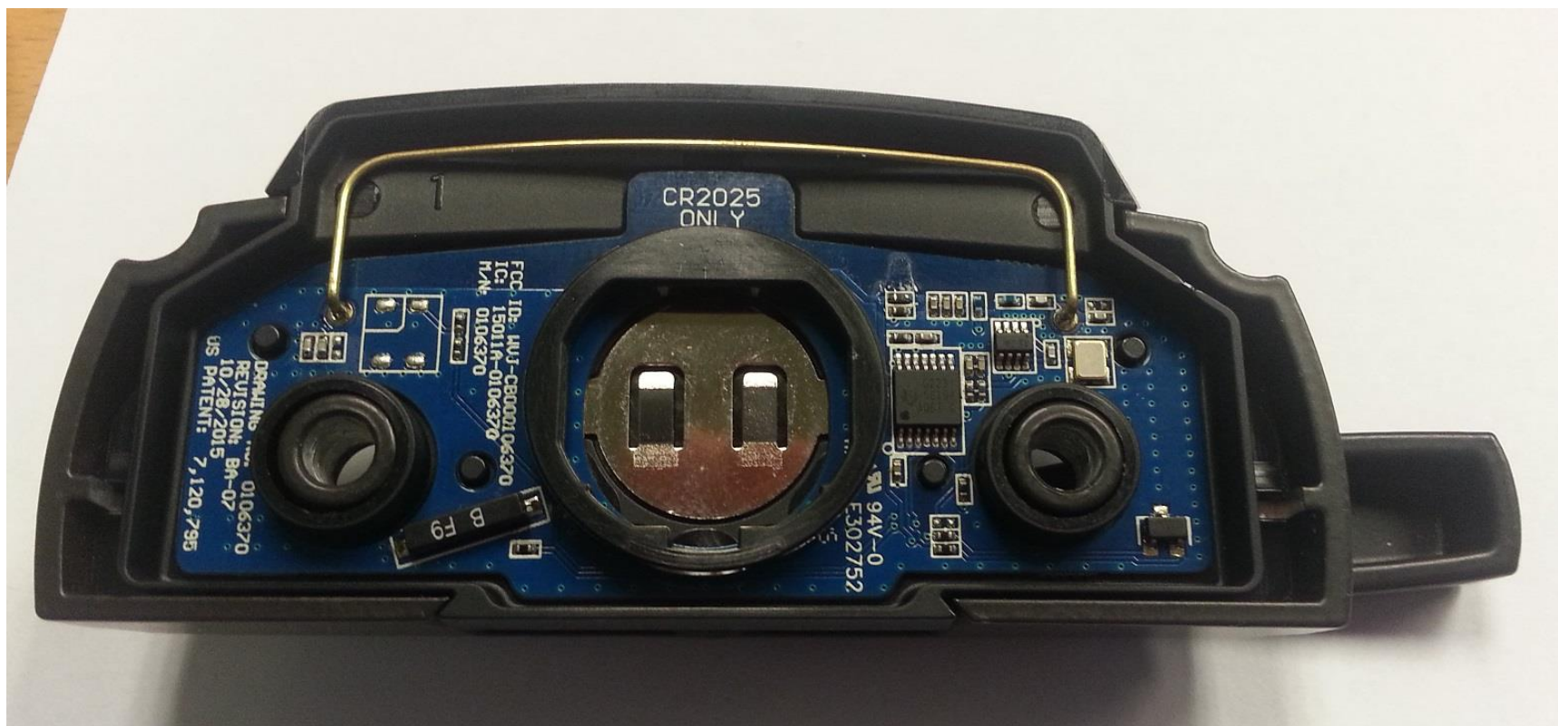
400-DH PHOTO – PCB in Carrier with Cover FRONT
