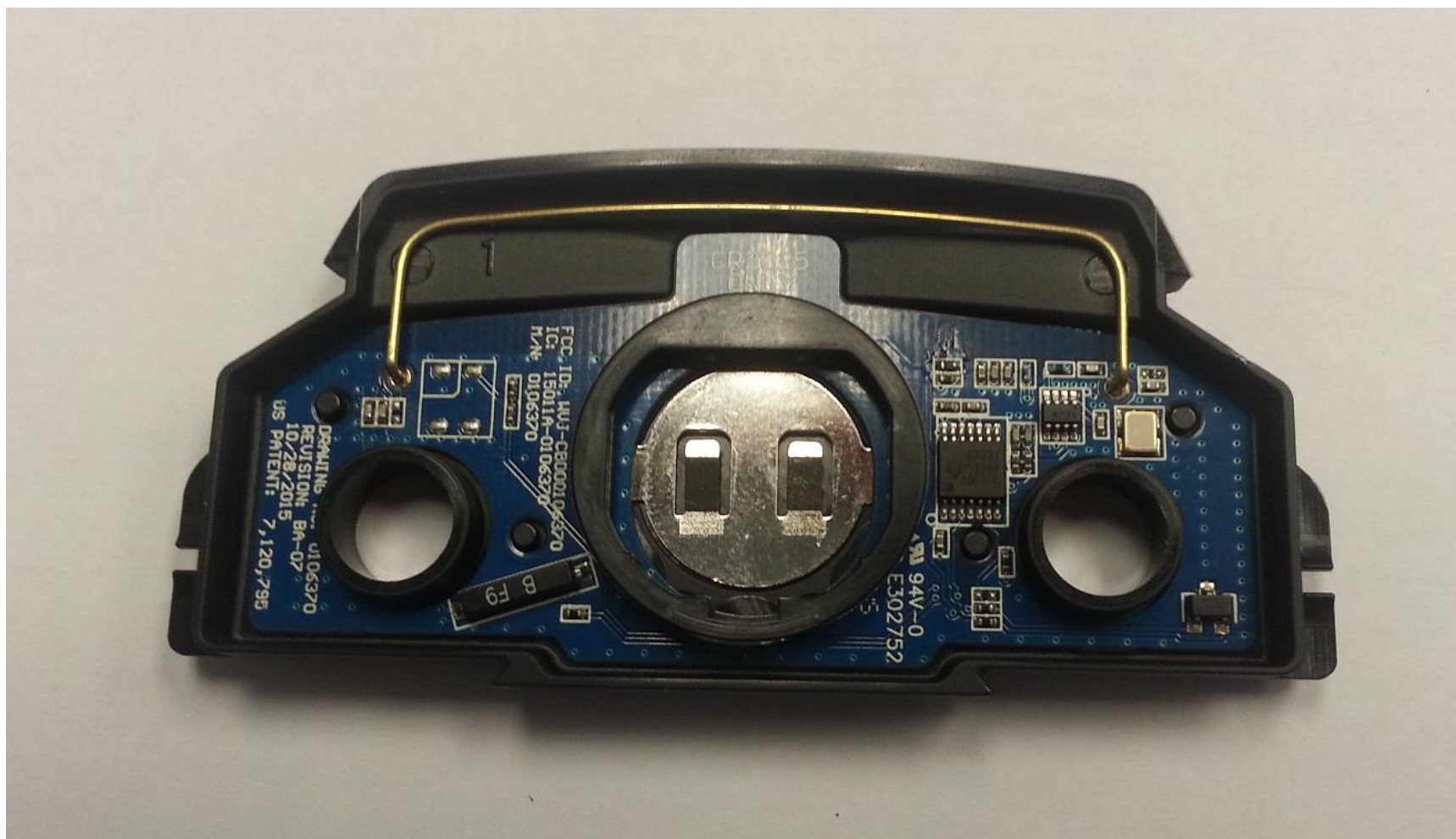
400-DH PHOTO - PCB in Carrier FRONT
