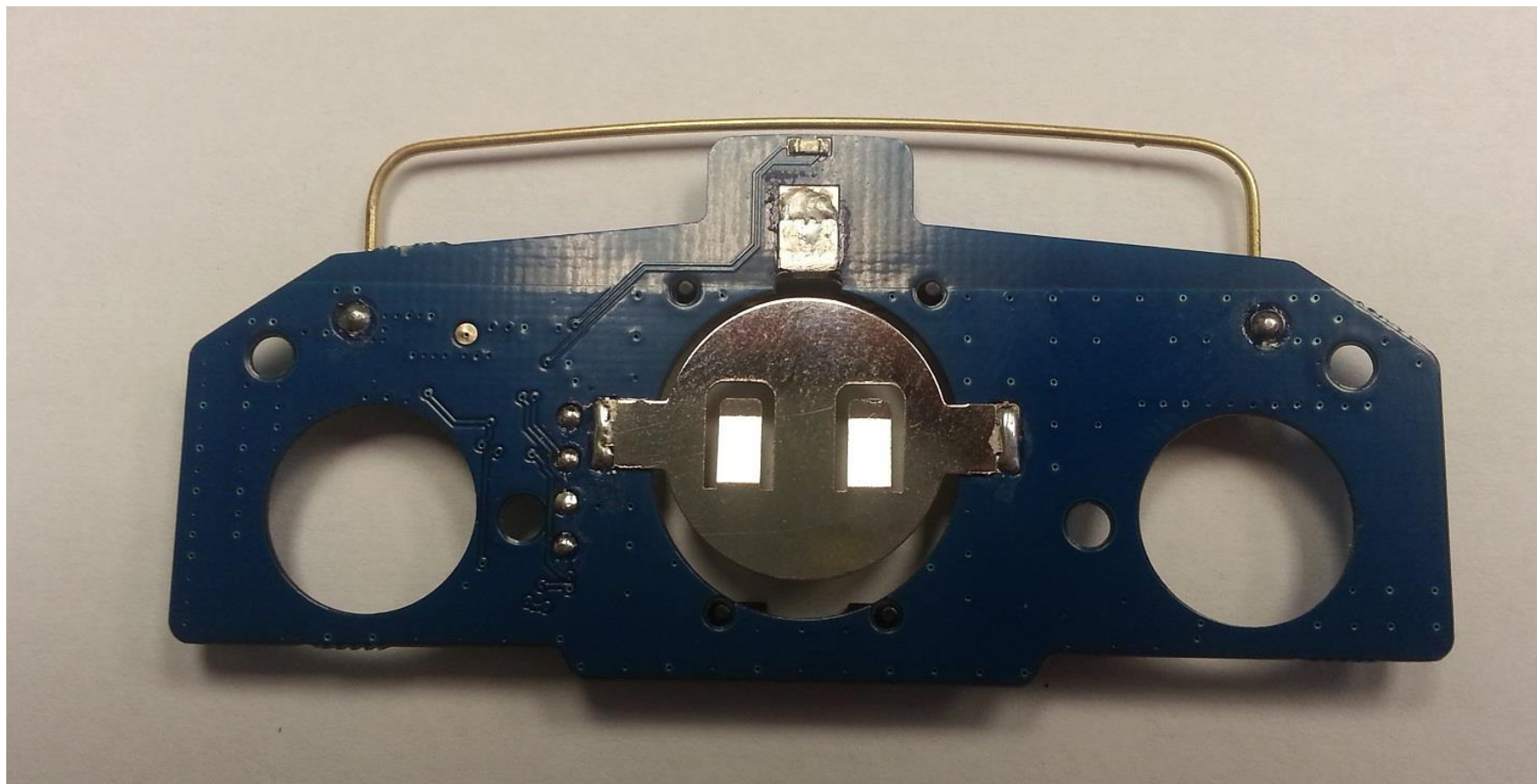
400-DH PHOTO – PCB BACK
