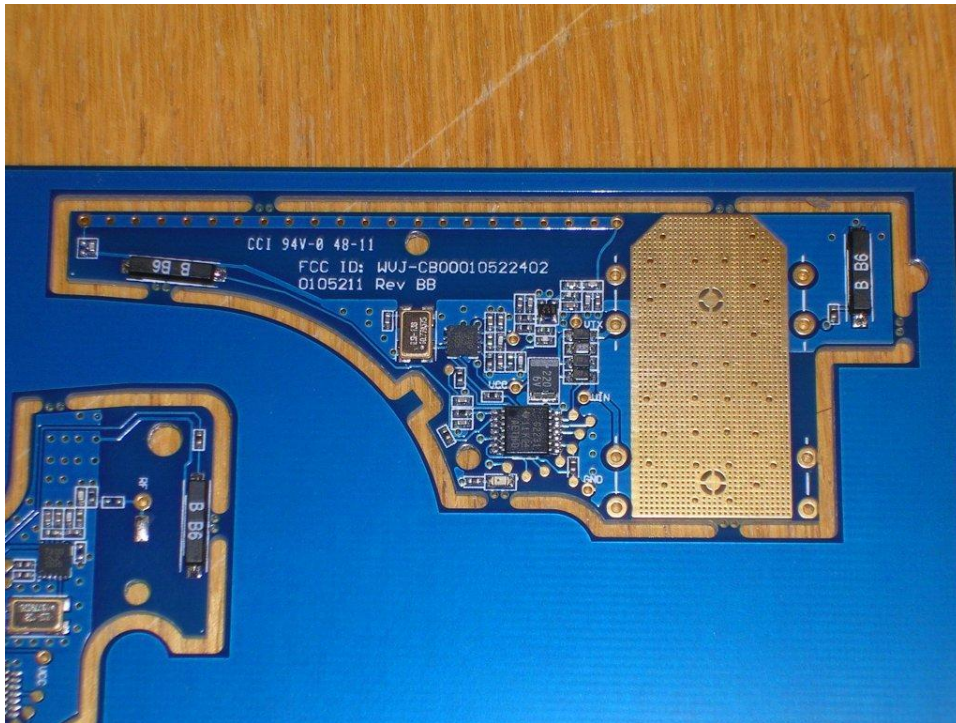
Figure 2 CSMT rev BB Internal battery up pcb
