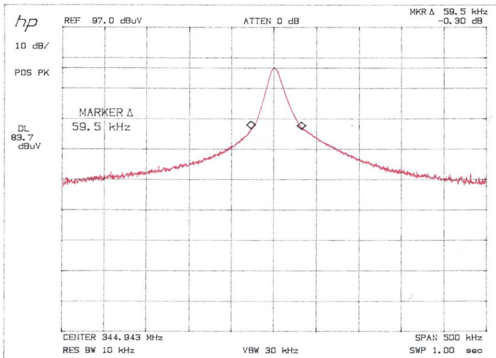
20dB Bandwidth Test: CSMT Sensor
