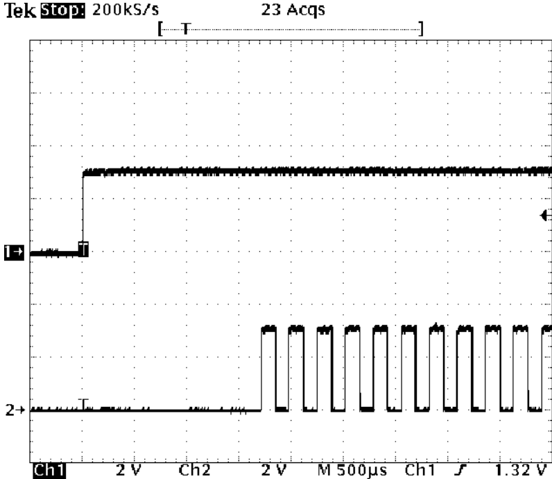
Figure 3 Transmitted Data Packet, 0.5 ms/div
