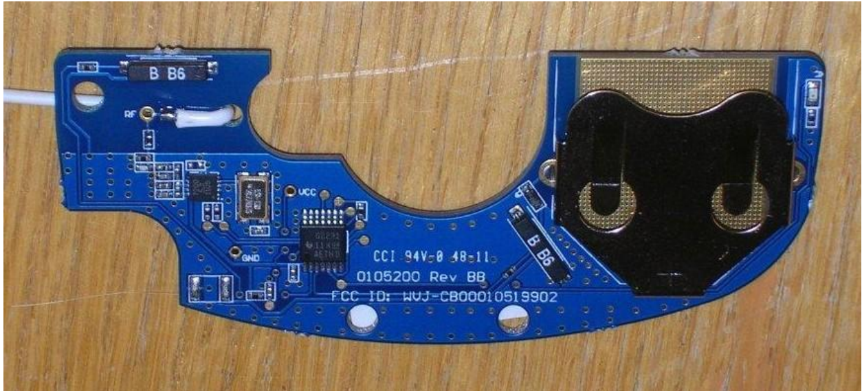
Figure 2 DH rev BB internal battery up pcb assembly
