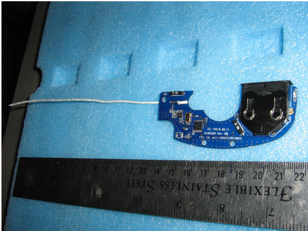
Figure 2 DH rev BB external battery up pcb assembly with battery housing
