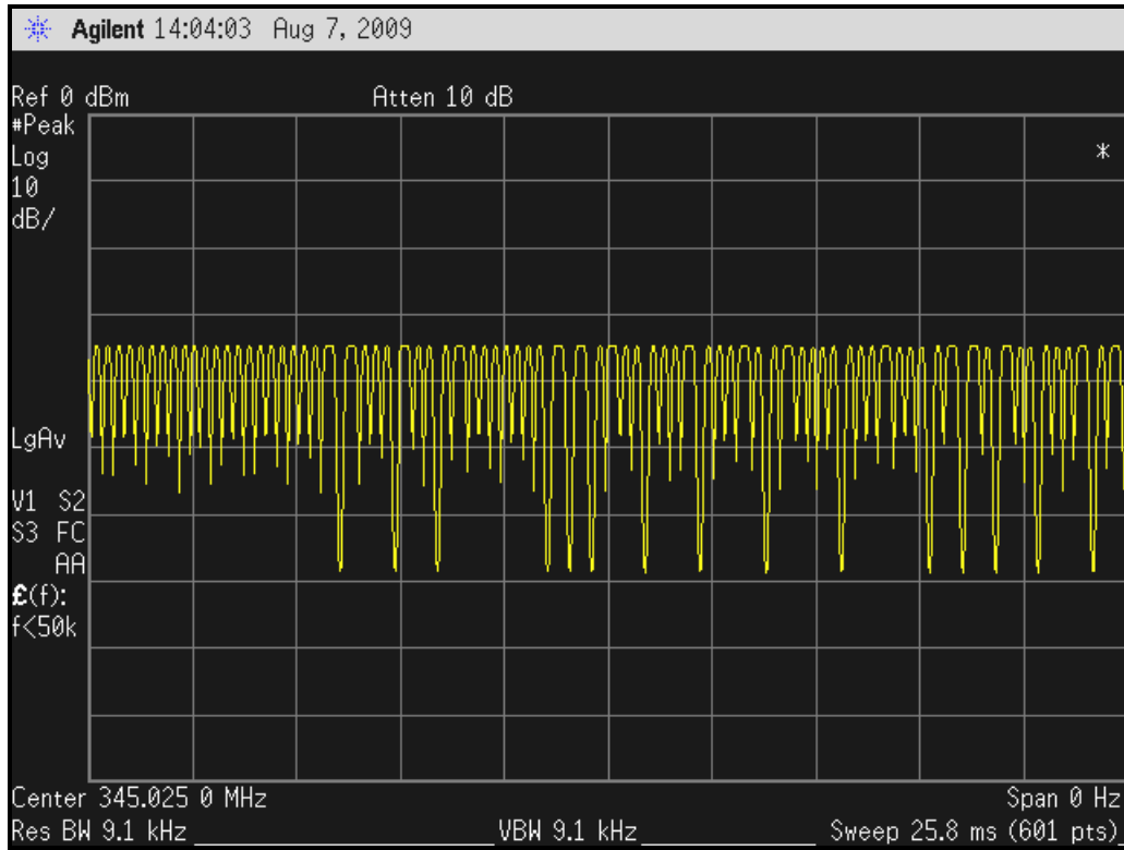
Plot 3-2: Total Pulse on Time within 25.8 ms Pulse Train Less than 50%
