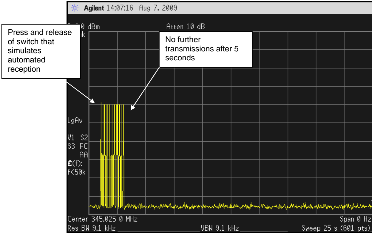
Plot 4-1: Transmitter Deactivation
