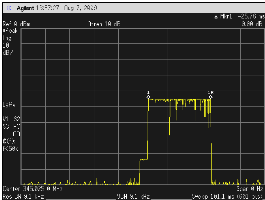
Plot 3-1: Total Pulse Train Length – 25.78 ms
