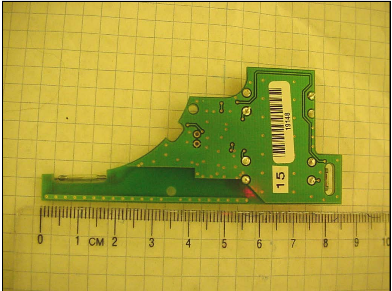
Photograph 6: Bottom of PCB
