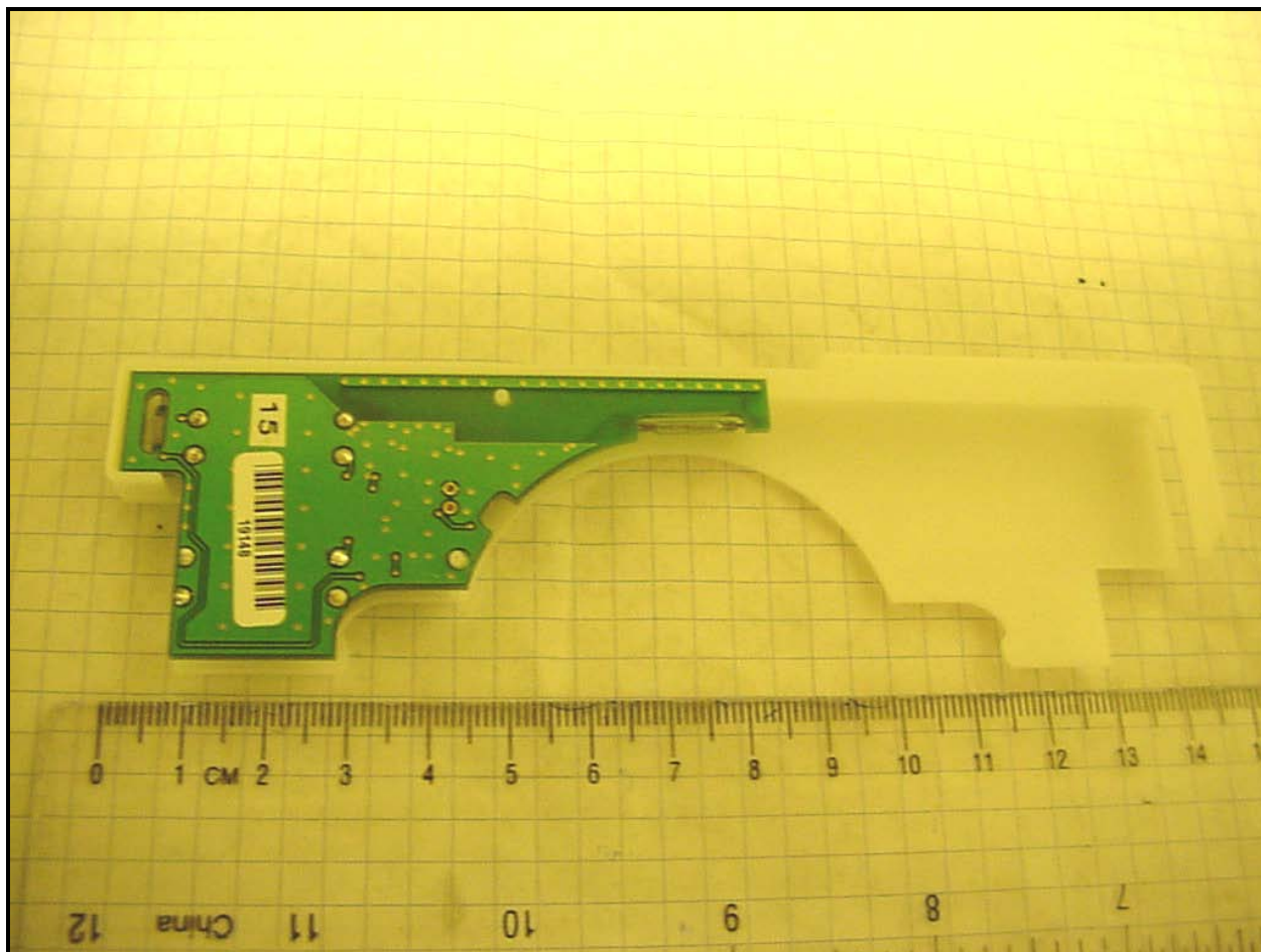
Photograph 4: External Photo Showing PCB
