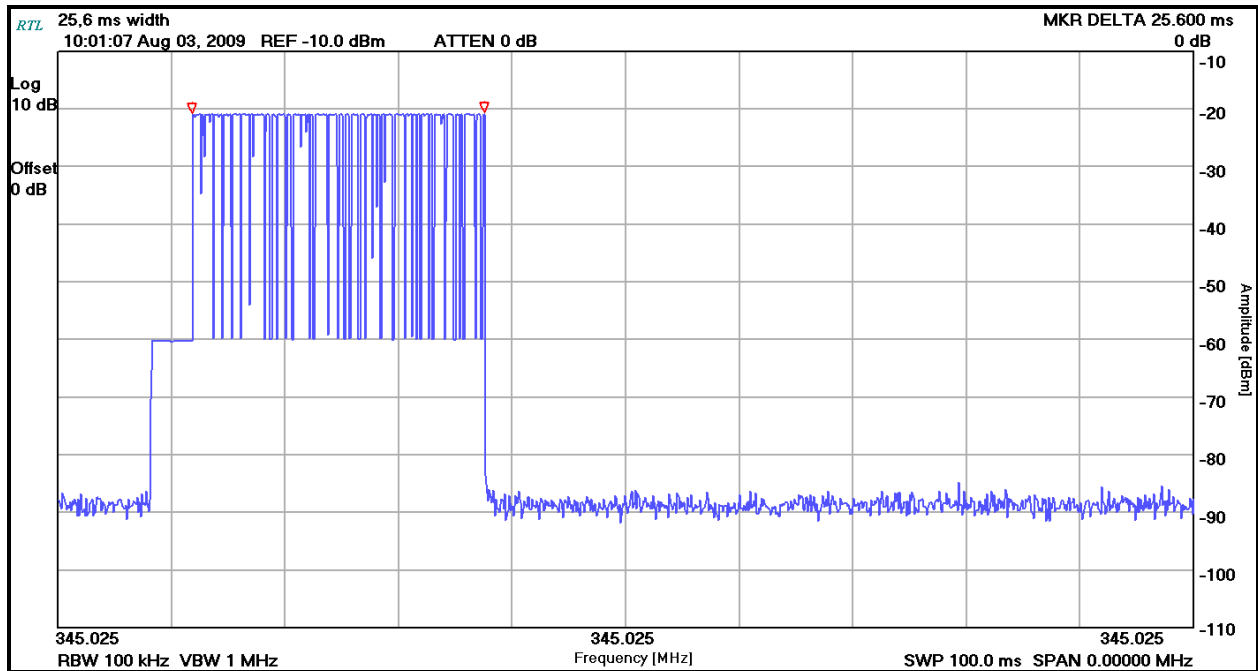
Plot 3-1: Total Pulse Train Length – 25.6 ms
