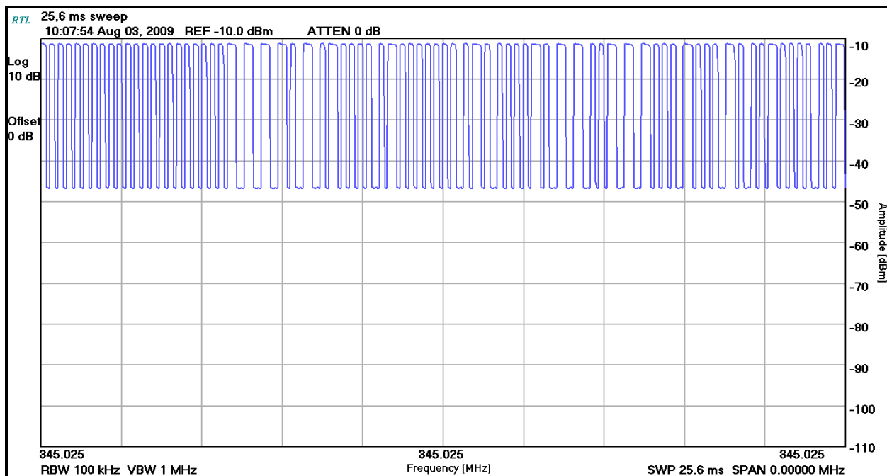
Plot 3-2: Total Pulse on Time within 25.6 ms Pulse Train Less than 50%
