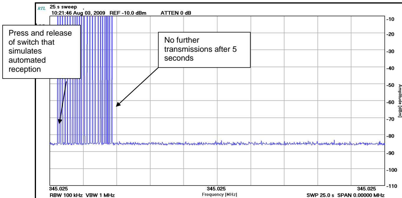
Plot 4-1: Transmitter Deactivation
