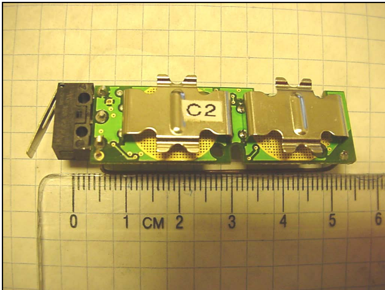
Photograph 5: PCB Back
