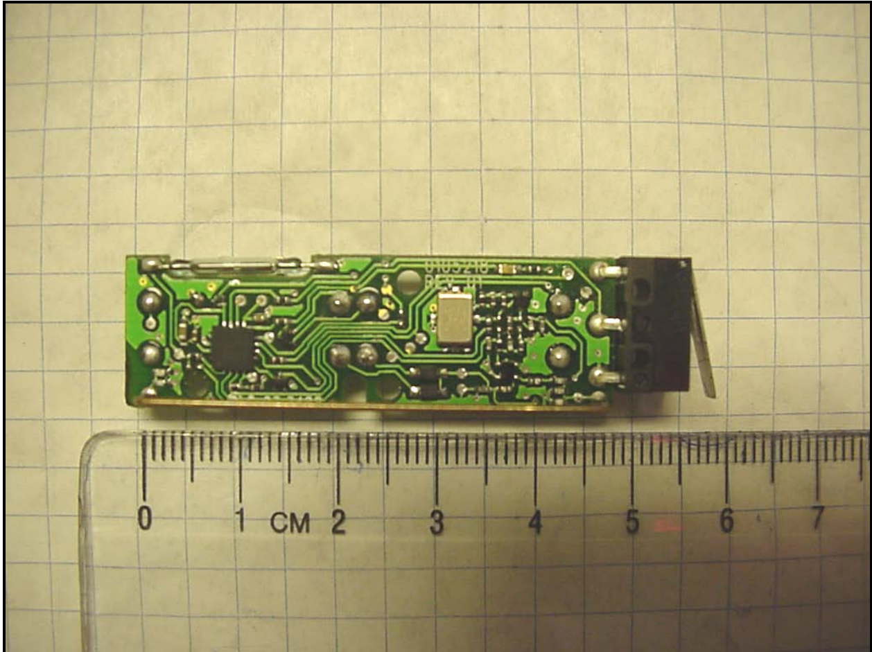
Photograph 4: PCB Front
