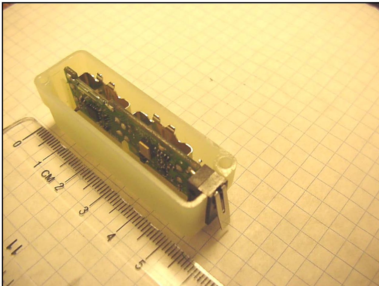
Photograph 3: EUT
