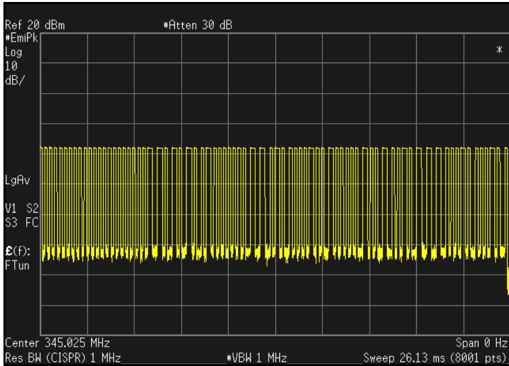
Plot 3-2: Total Pulse on Time within 25.8 ms Pulse Train Less than 50%
