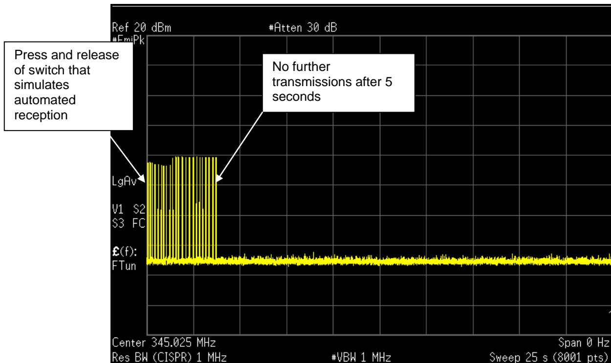
Plot 4-1: Transmitter Deactivation
