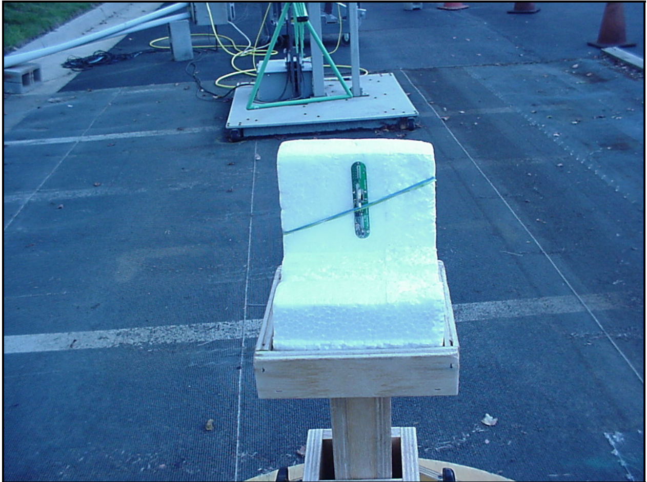
Photograph 1: Radiated Emissions
