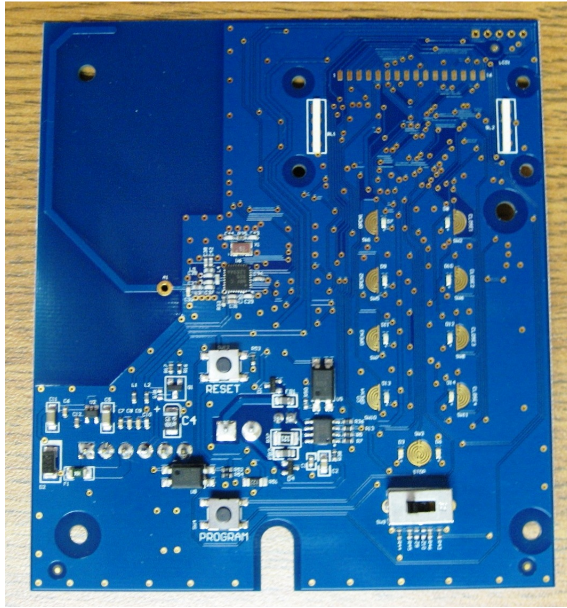
Circuit Board Side 1 with Display Removed
