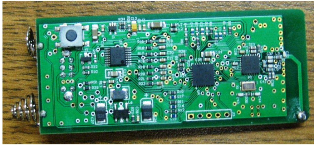
Circuit Board Side 2
