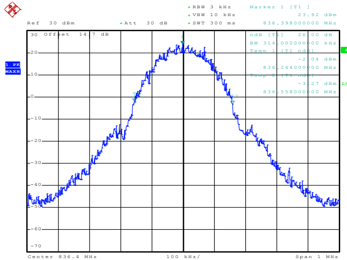
26dB Bandwidth Plot on Channel 189
