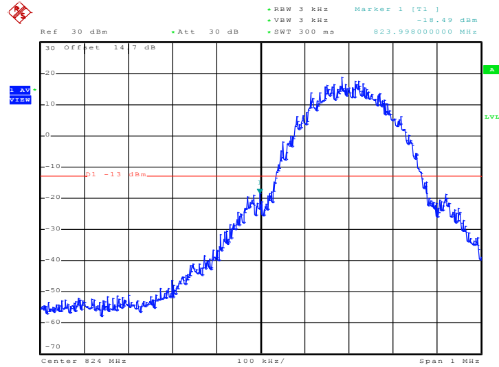
Lower Band Edge Plot on Channel 128
