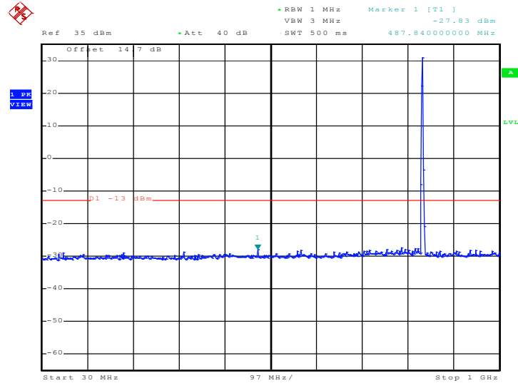
Conducted Emission Plot between 30MHz ~ 1GHz
