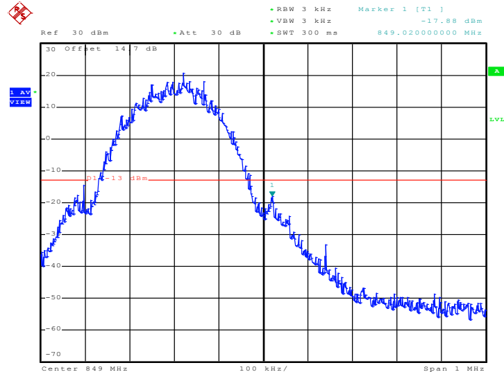
Higher Band Edge Plot on Channel 251
