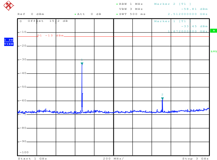
Conducted Emission Plot between 1GHz ~ 3GHz
