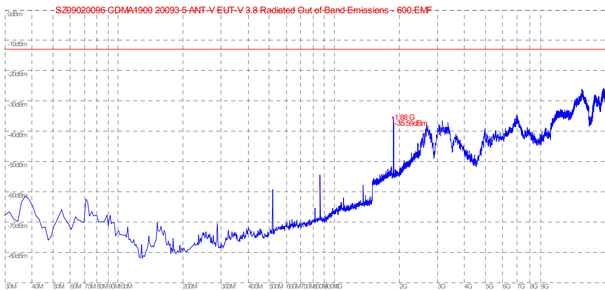
(Plot D: CDMA 1900MHz Channel = 600, Test Antenna Vertical)
