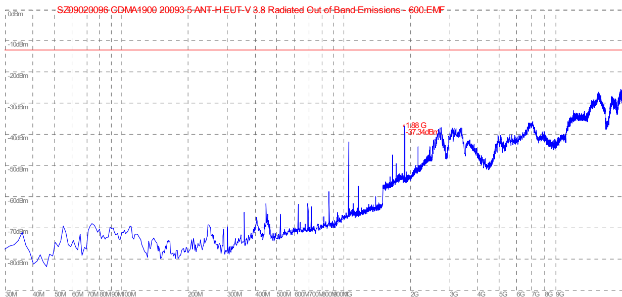
(Plot C: CDMA 1900MHz Channel = 600, Test Antenna Horizontal)
