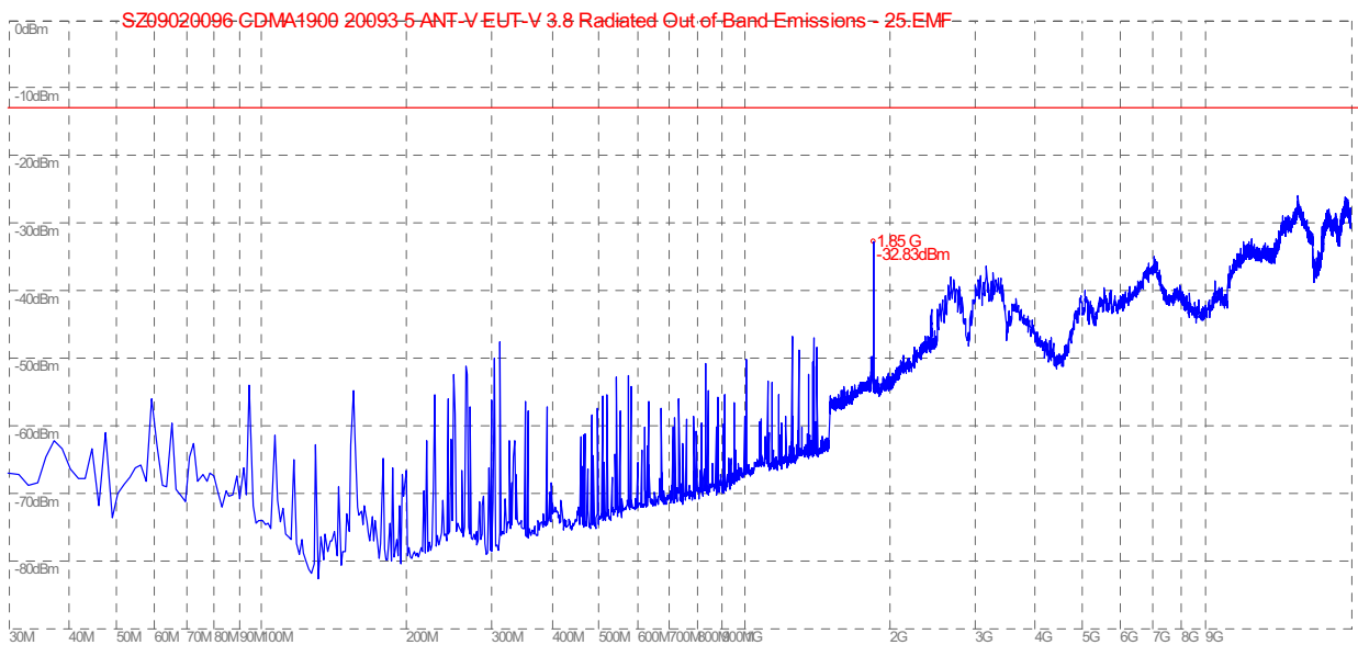
(Plot B: CDMA 1900MHz Channel = 25, Test Antenna Vertical)
