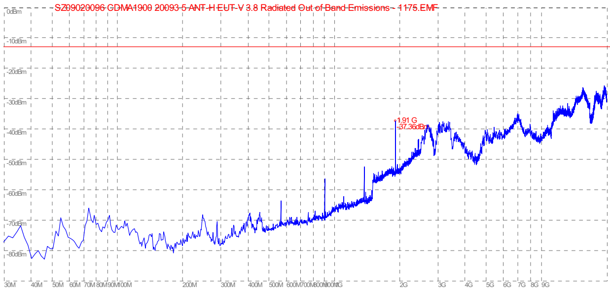
(Plot E: CDMA 1900MHz Channel = 1175, Test Antenna Horizontal)
