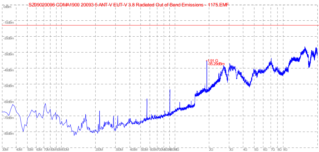
(Plot F: CDMA 1900MHz Channel = 1175, Test Antenna Vertical)
