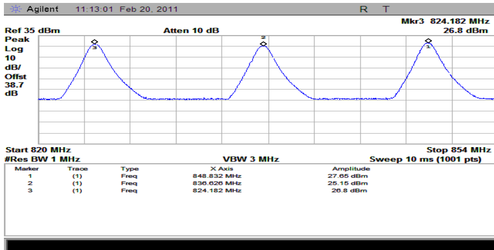
(Plot A: GSM 850MHz Channel = 128,190,251)
