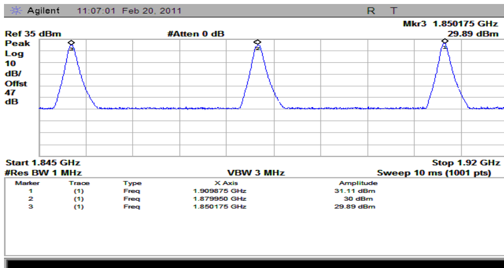
(Plot B: GSM 1900MHz Channel = 512, 661, 810)
