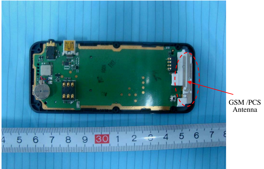
EUT – Inside View
