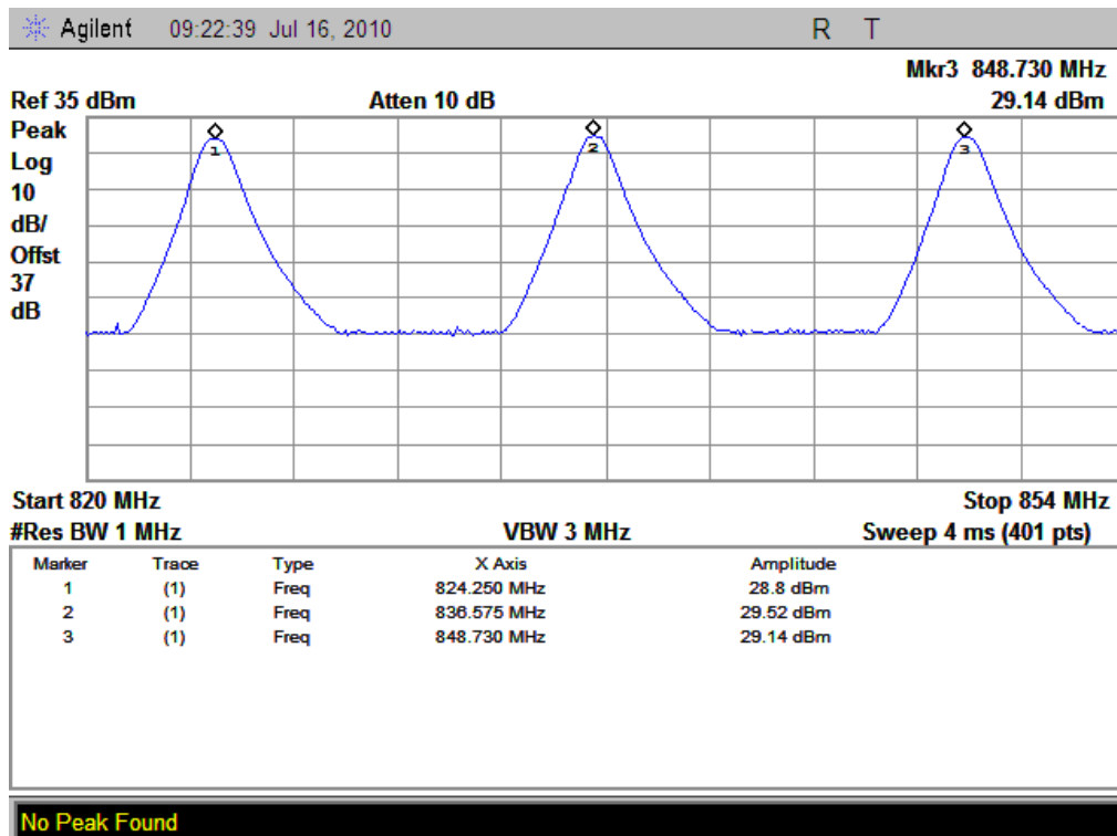
(Plot C: GPRS-2TX 850MHz Channel = 128, 190, 251)
