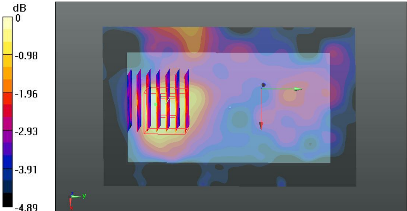
0 dB = 0.0121 \text{ W/kg}
