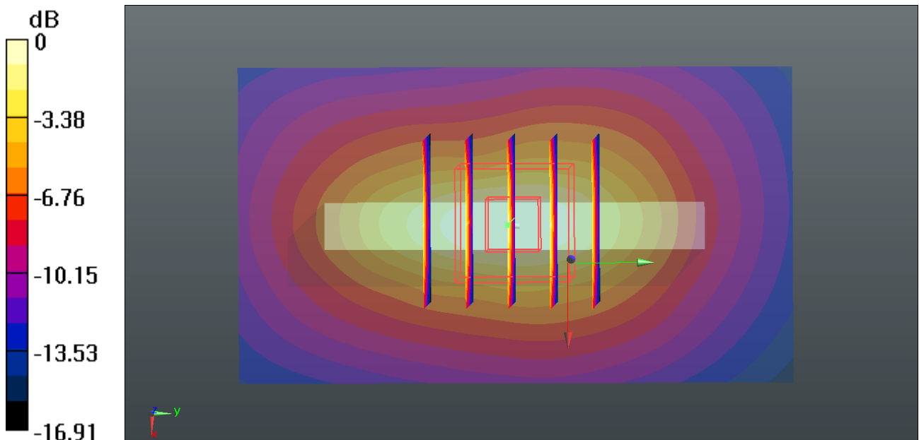
0 dB = 0.686 W/kg
