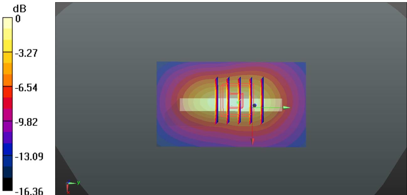
0 dB = 0.632 W/kg
