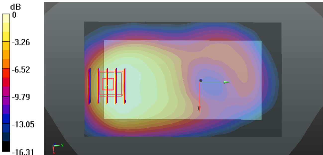
0 dB = 0.737 W/kg
