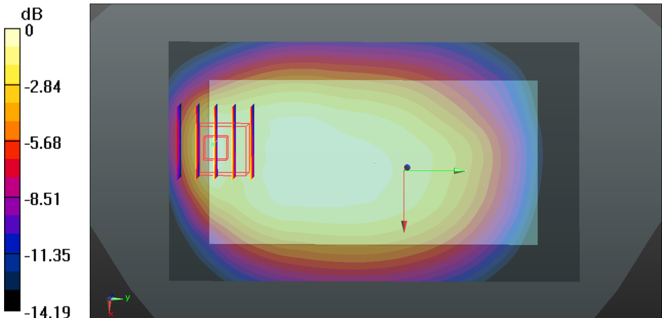
0 dB = 0.712 W/kg
