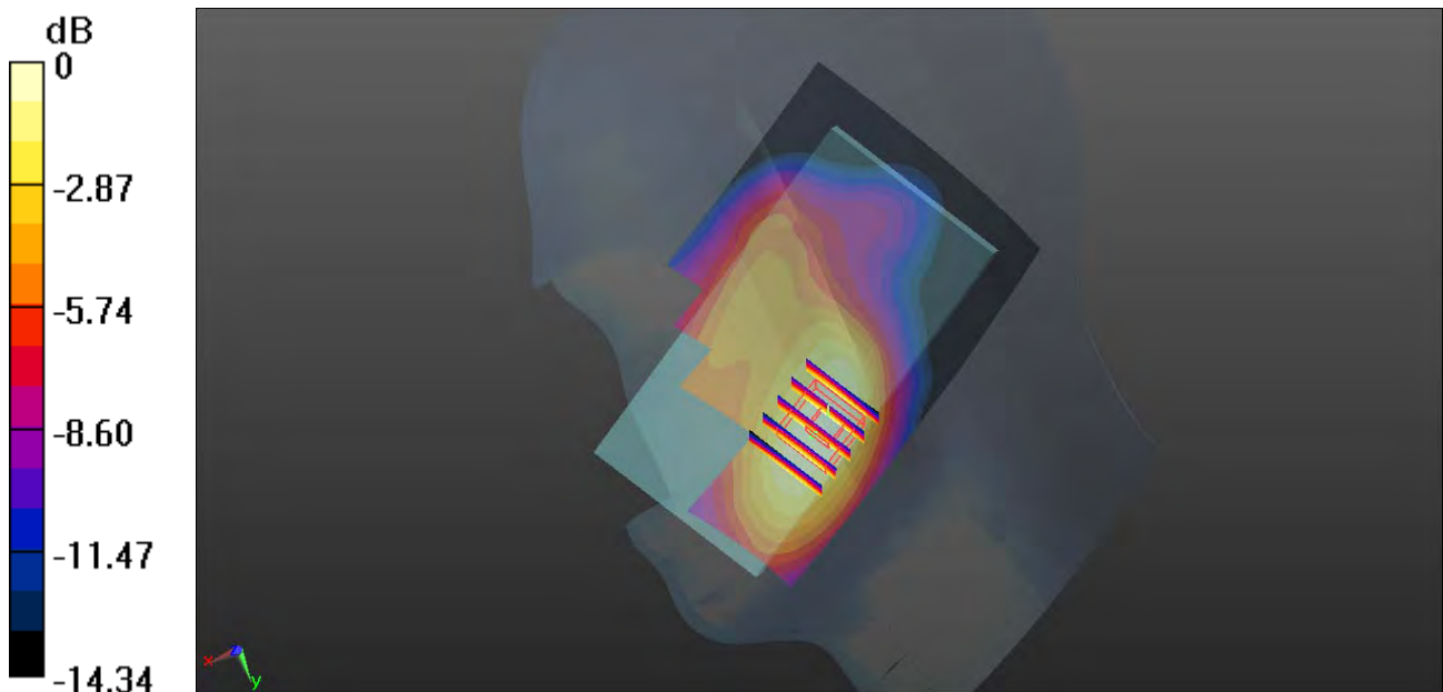
0 dB = 0.309 W/kg
