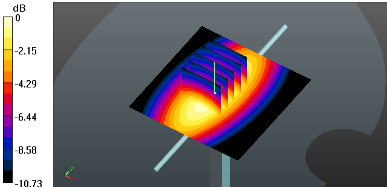
0 dB = 2.99 W/kg
