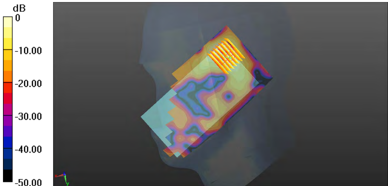
0 dB = 0.346 W/kg
