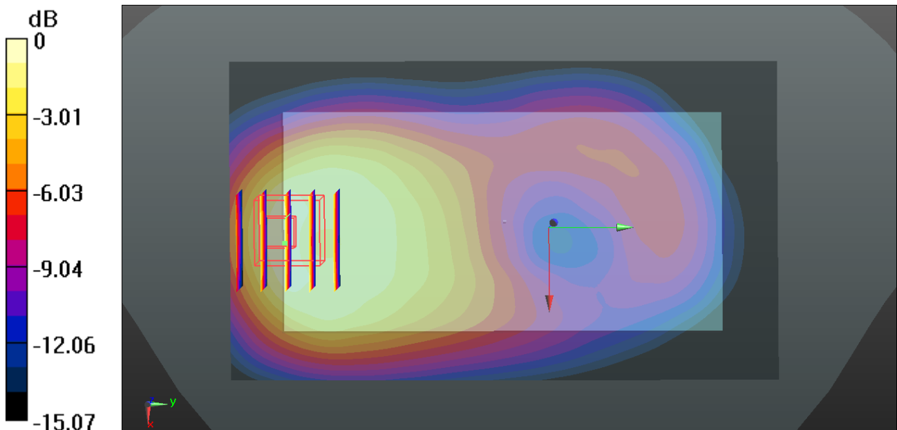
0 dB = 0.678 W/kg
