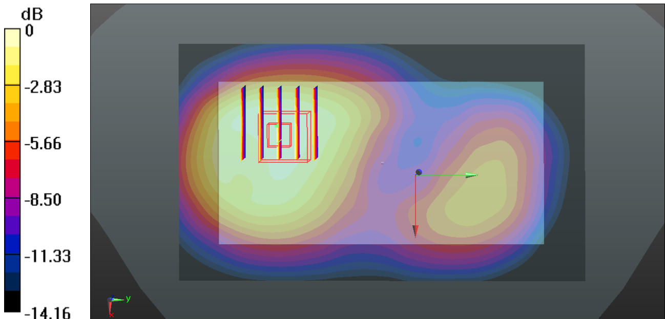
0 dB = 0.561 W/kg
