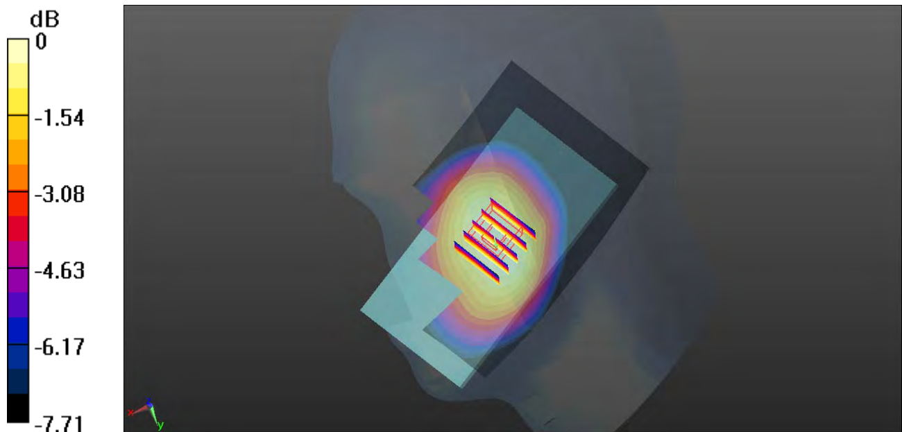
0 dB = 0.167 W/kg
