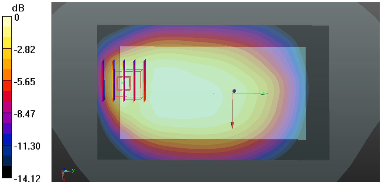
0 dB = 0.320 W/kg
