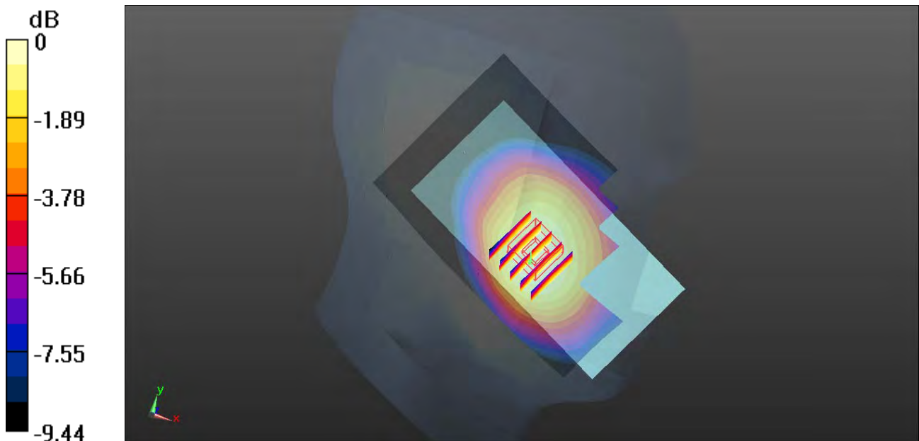
0 dB = 0.494 W/kg
