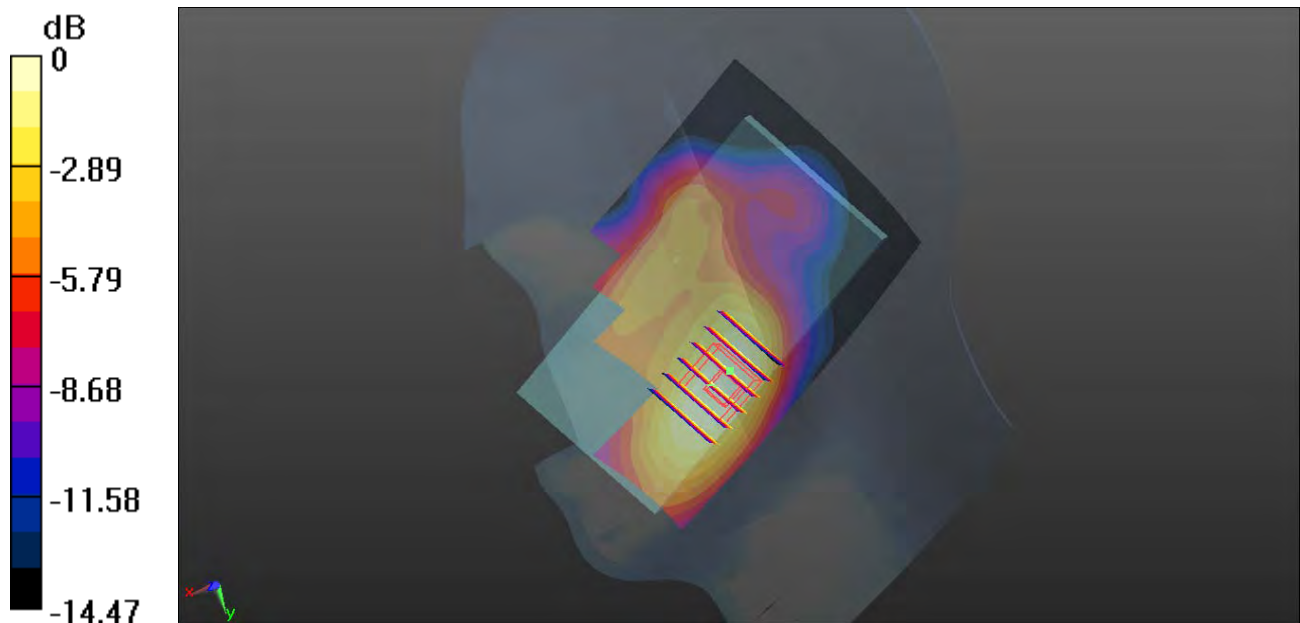
0 dB = 0.269 W/kg
