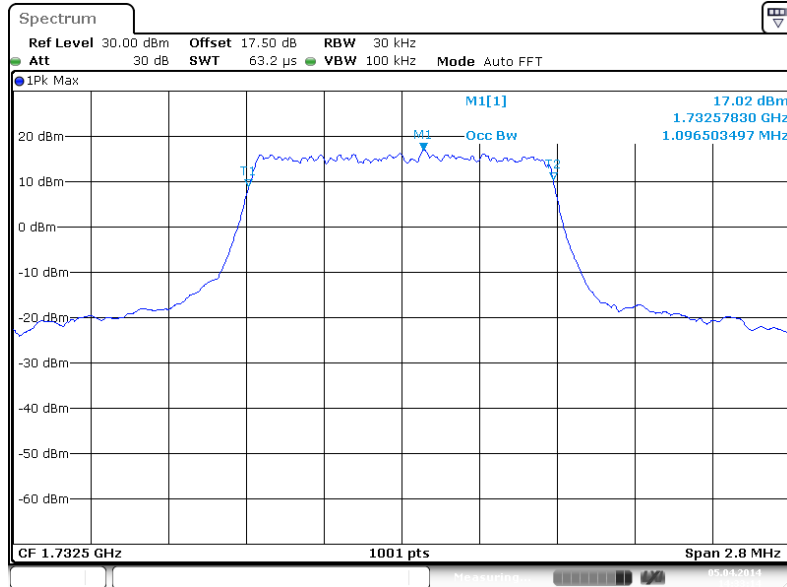
99% Occupied Bandwidth Plot on Channel 20175
