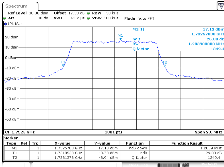
26dB Bandwidth Plot on Channel 20175
