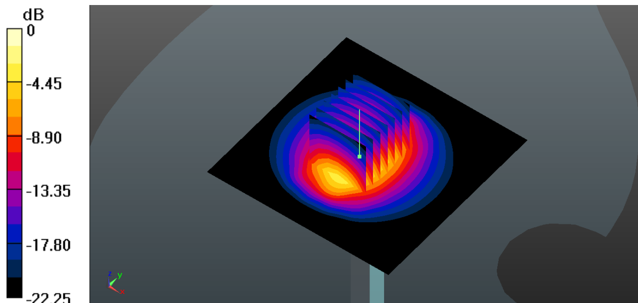
0 dB = 19.0 W/kg
