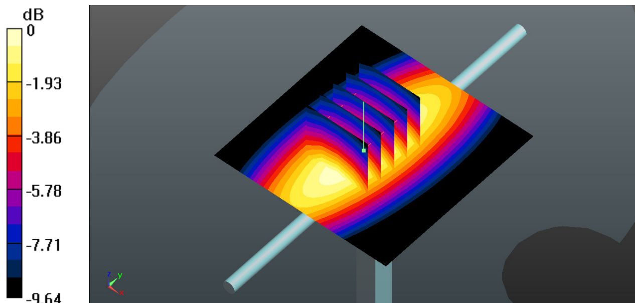
0 dB = 2.60 W/kg
