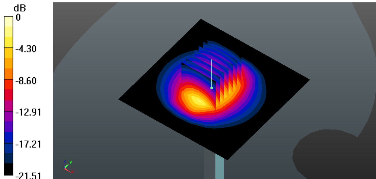
0 dB = 20.1 W/kg
