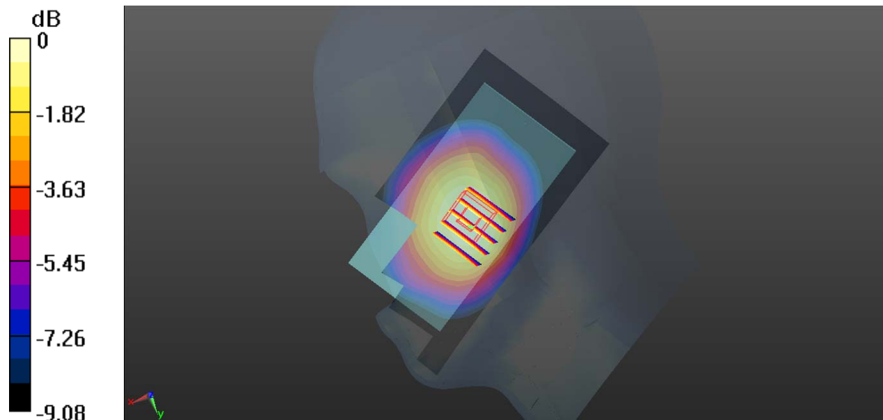
0 dB = 0.615 W/kg
