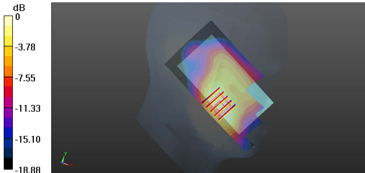
0 dB = 0.772 W/kg
