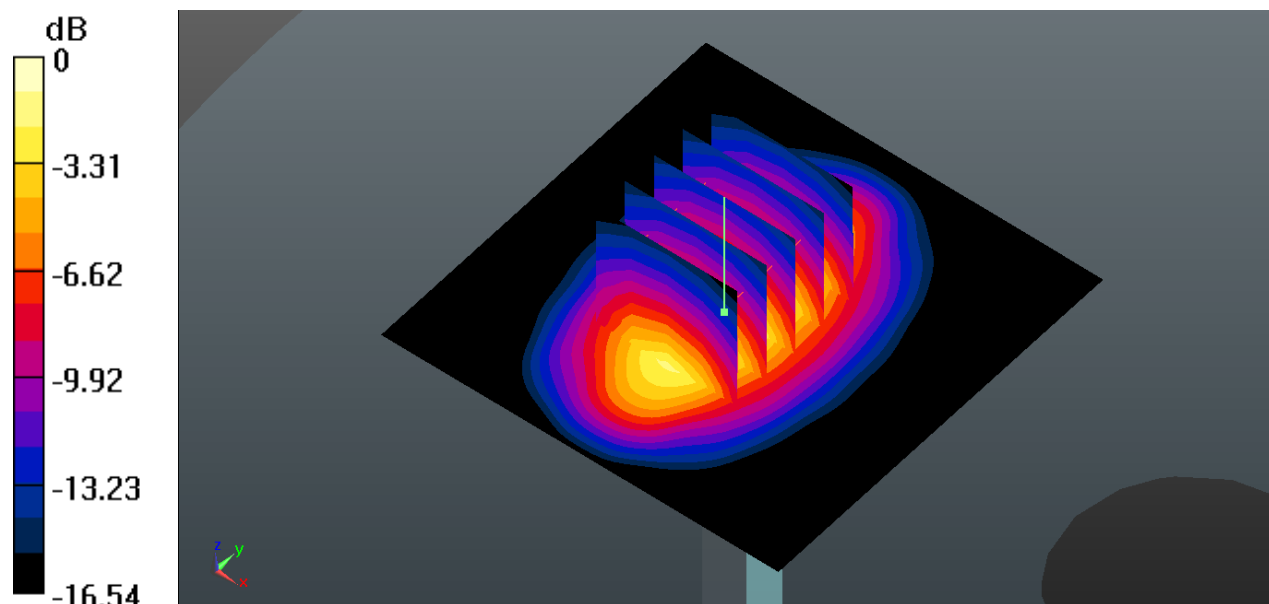
0 dB = 13.1 W/kg
