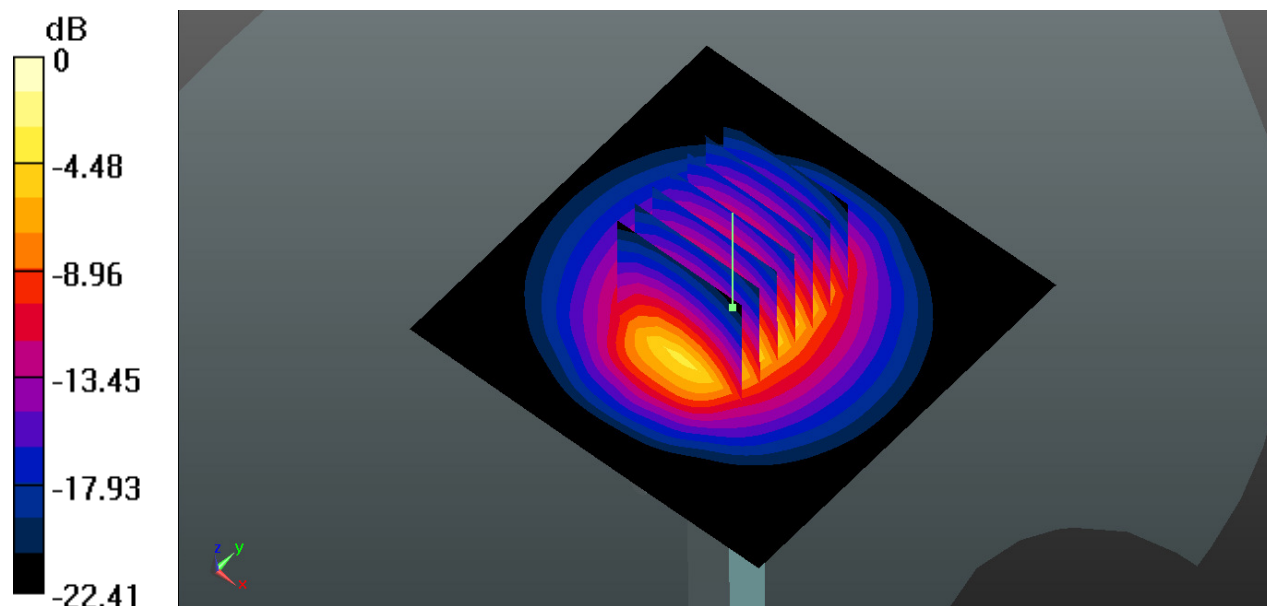
0 dB = 22.0 W/kg
