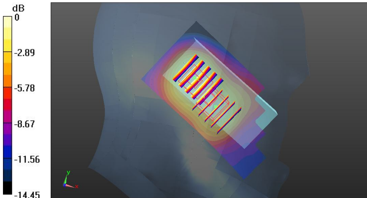
0 dB = 0.329 \text{ W/kg}
