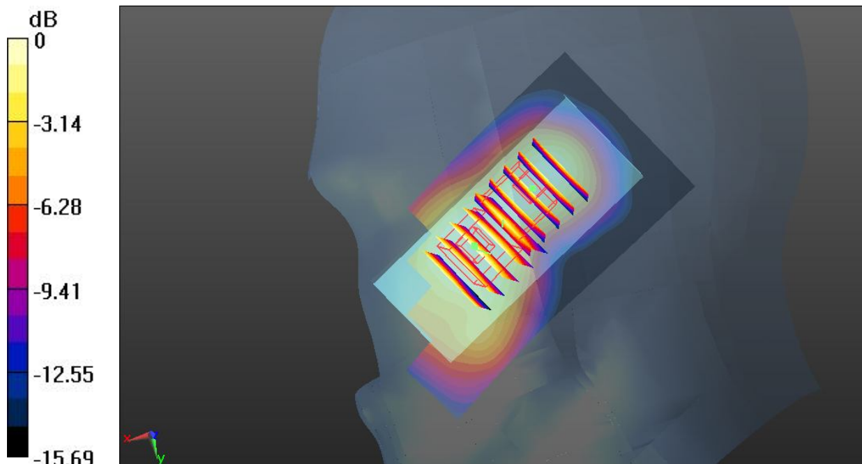
0 dB = 0.784 W/kg
