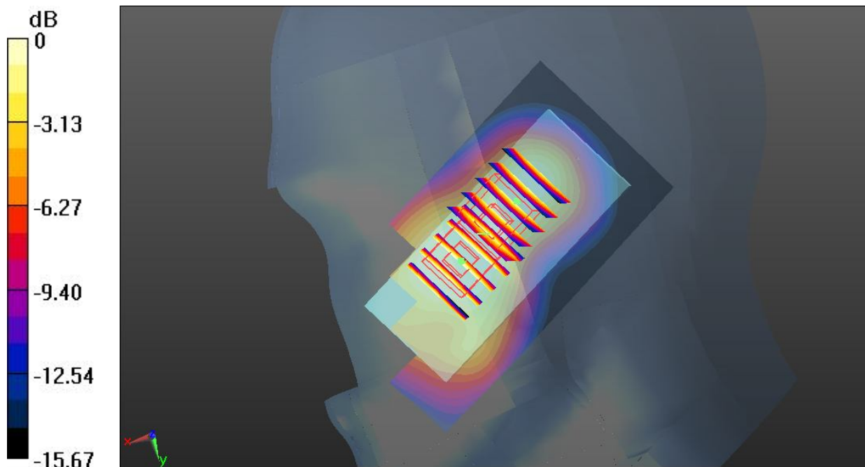
0 dB = 1.00 W/kg
