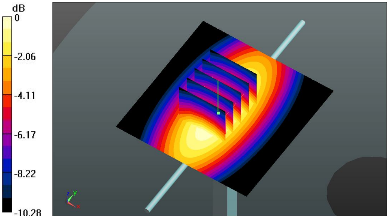
0 dB = 2.53 \text{ W/kg}
