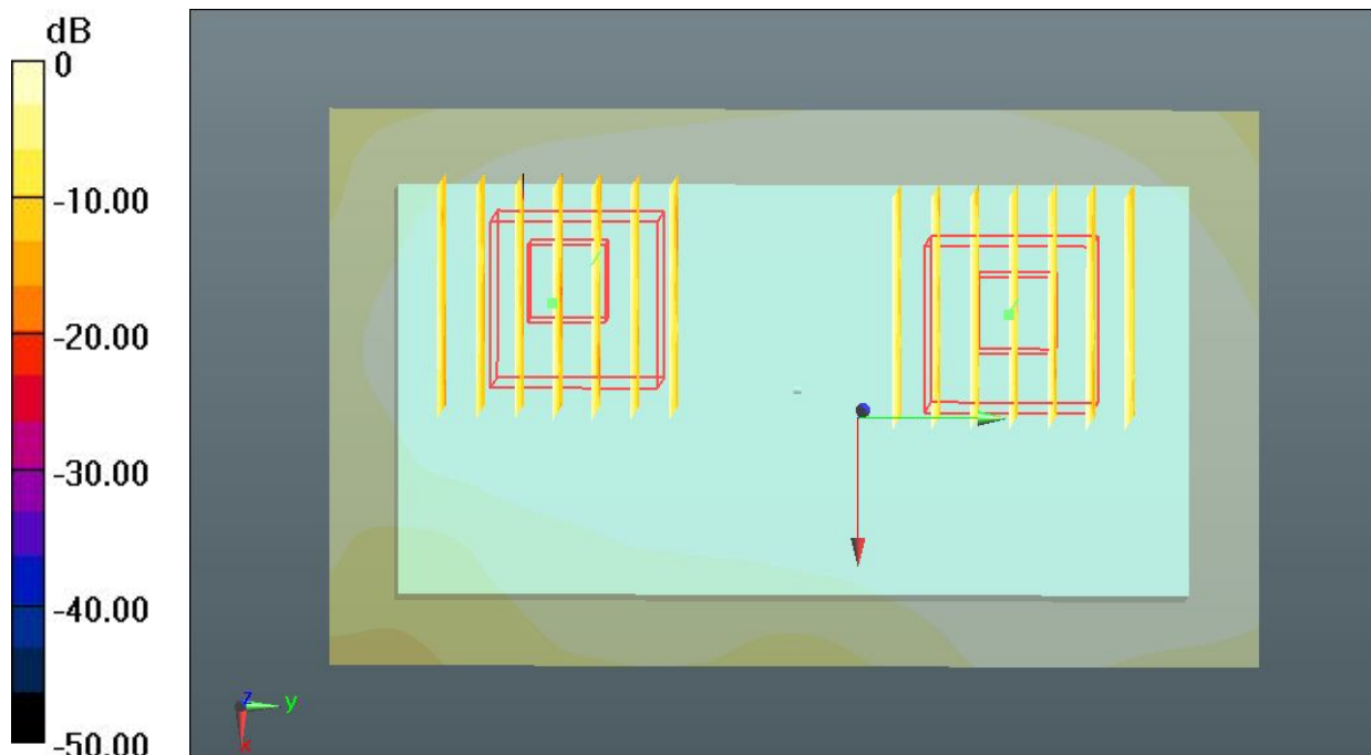
0 dB = 0.0259 W/kg
