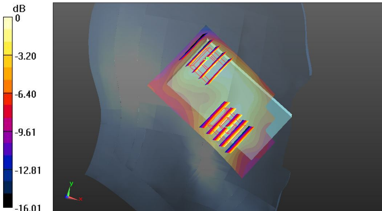
0 dB = 0.0530 W/kg
