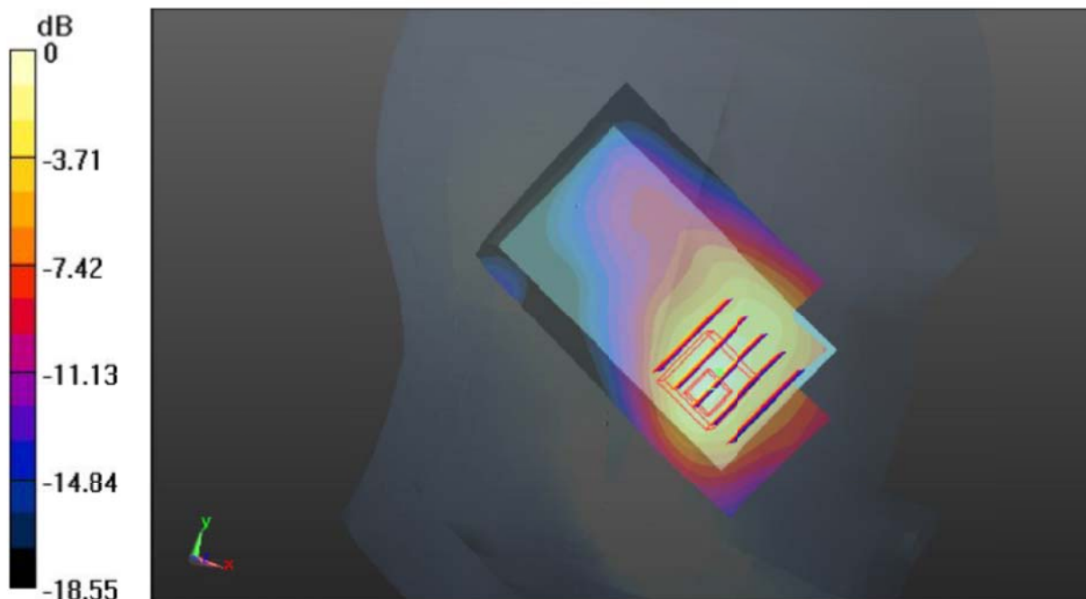
0 dB = 0.444 W/kg
