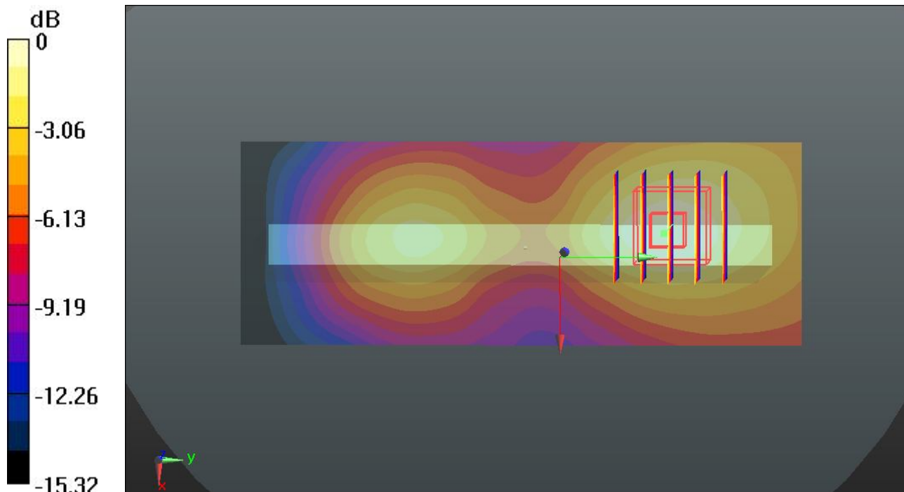
0 dB = 0.124 W/kg
