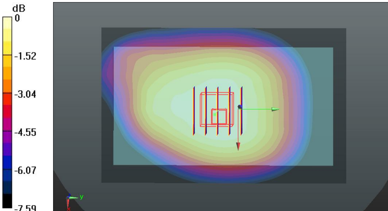
0 dB = 0.236 W/kg
