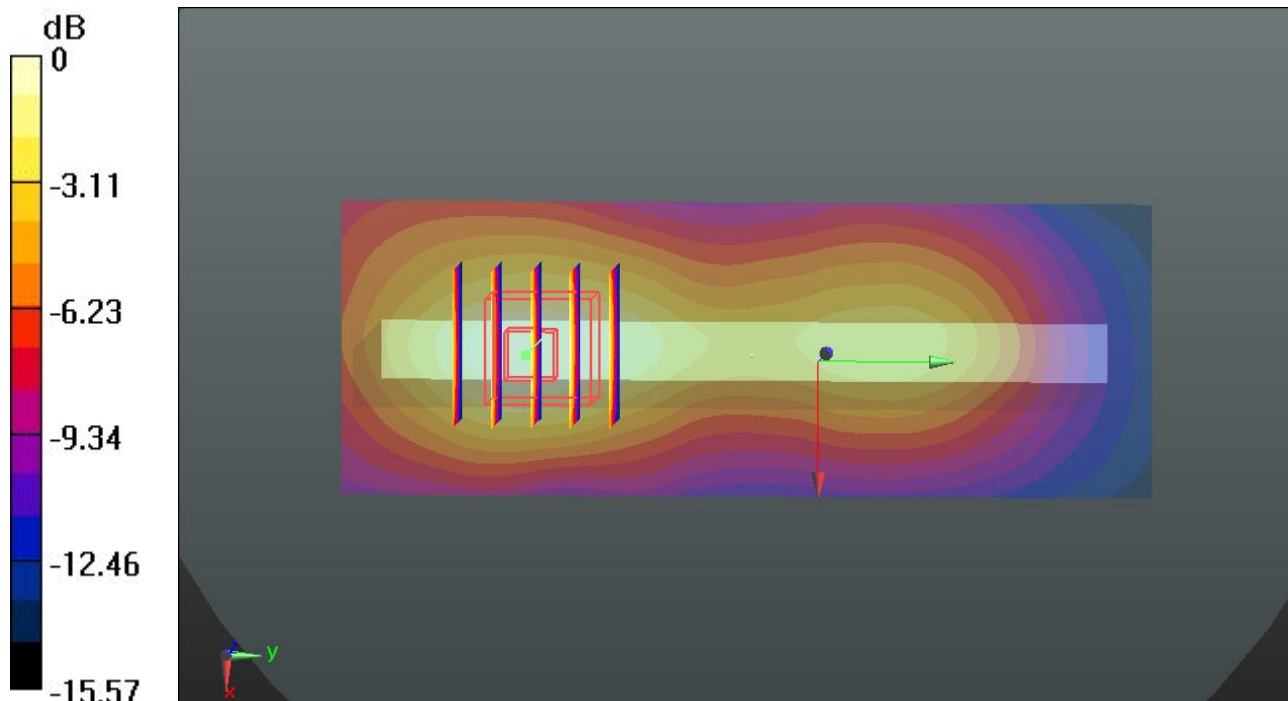
0 dB = 0.180 W/kg
