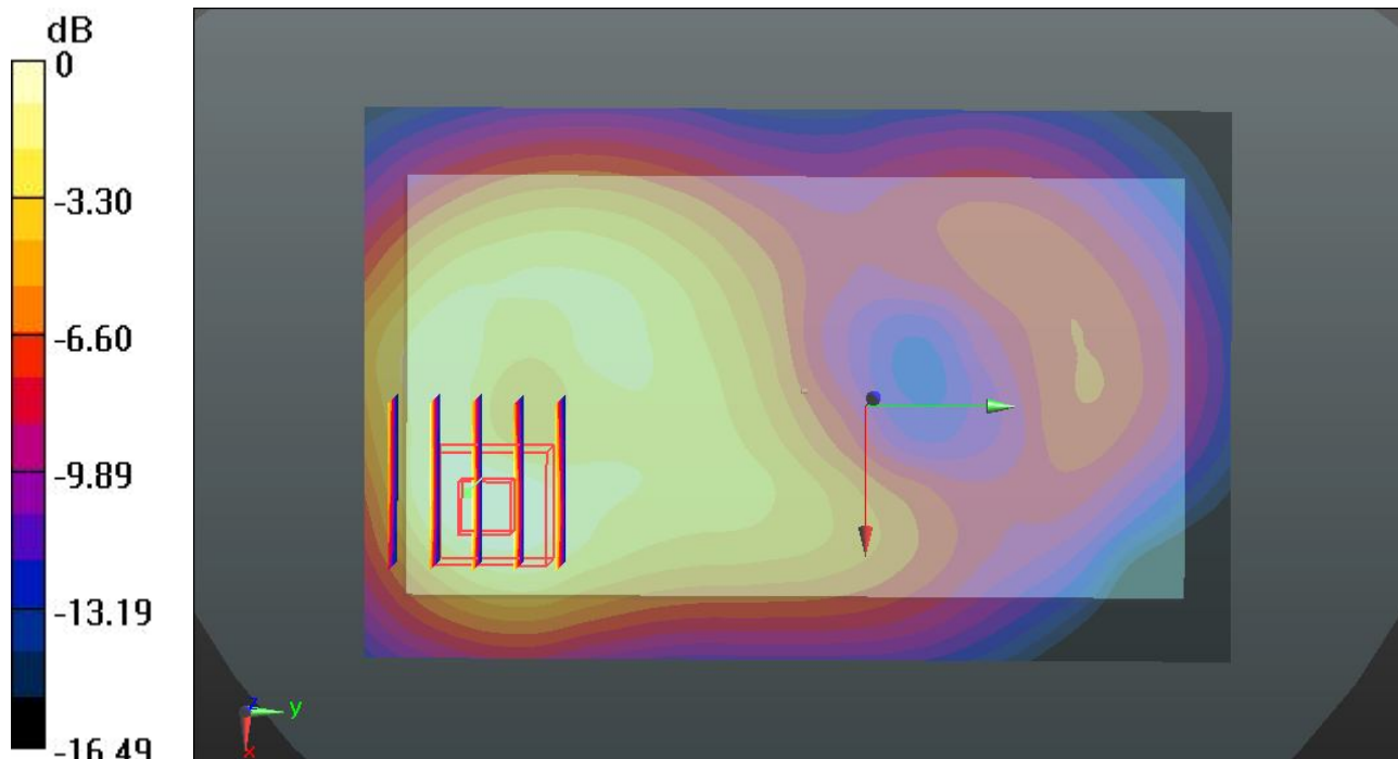
0 dB = 0.483 W/kg
