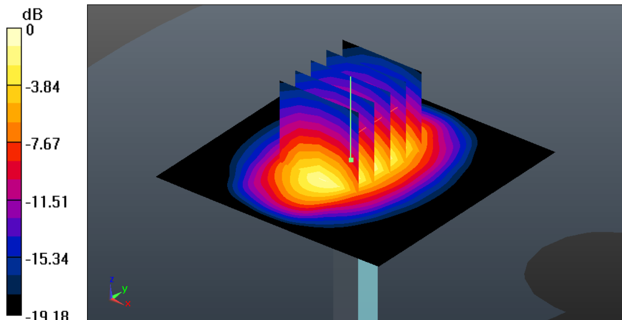
0 dB = 13.8 W/kg
