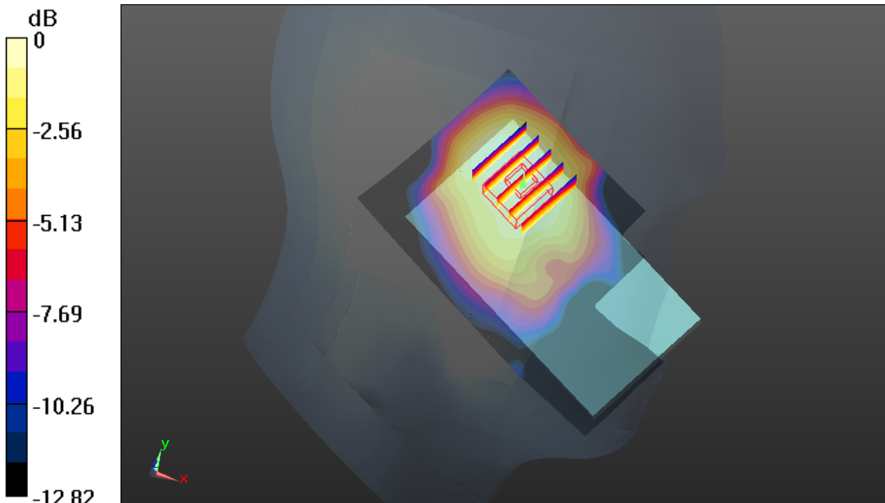
0 dB = 0.416 W/kg
