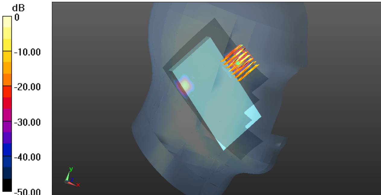
0 dB = 0.0969 W/kg
