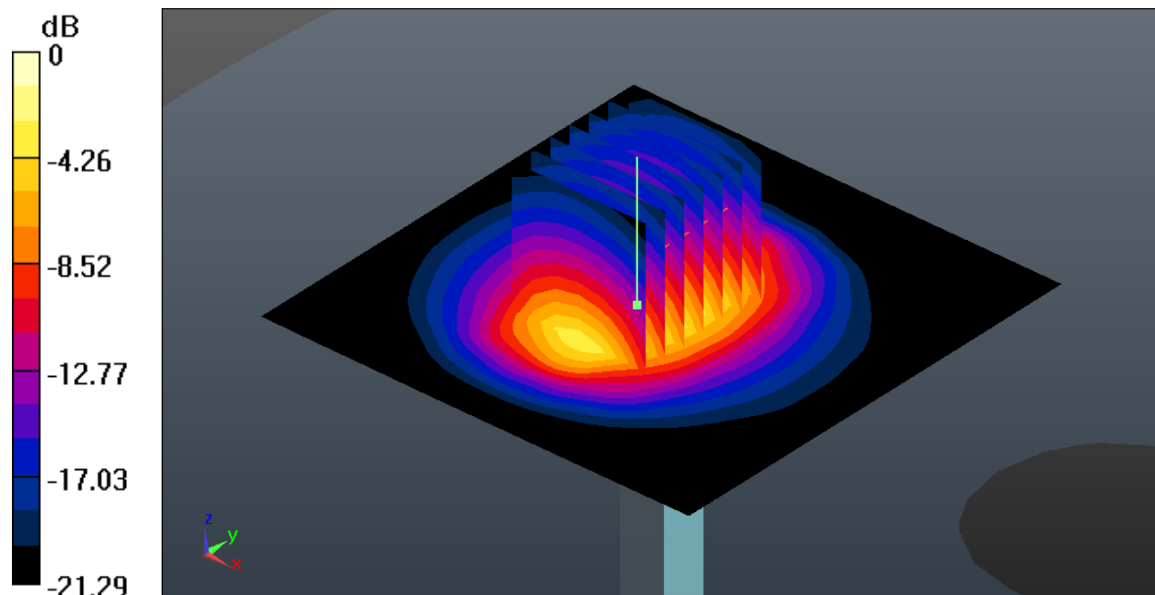
0 dB = 19.3 W/kg
