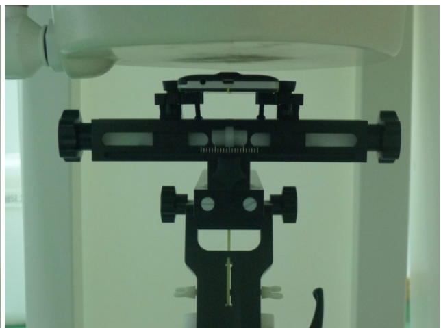
Back of the DUT with Phantom 1 cm
