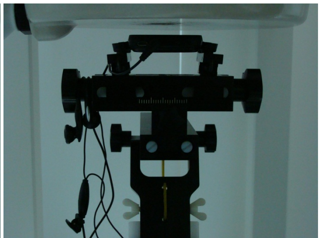
Front of the DUT with Earphone to phantom 1 cm gap
