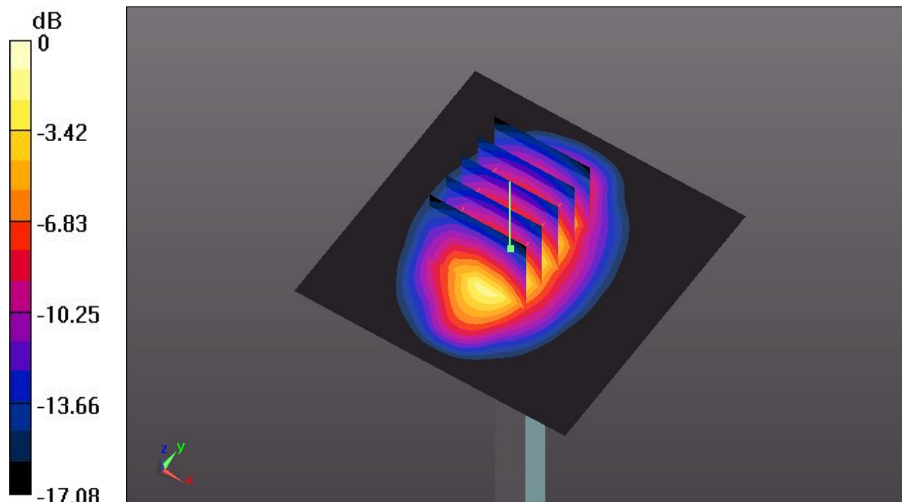
0 dB = 13.3 W/kg
