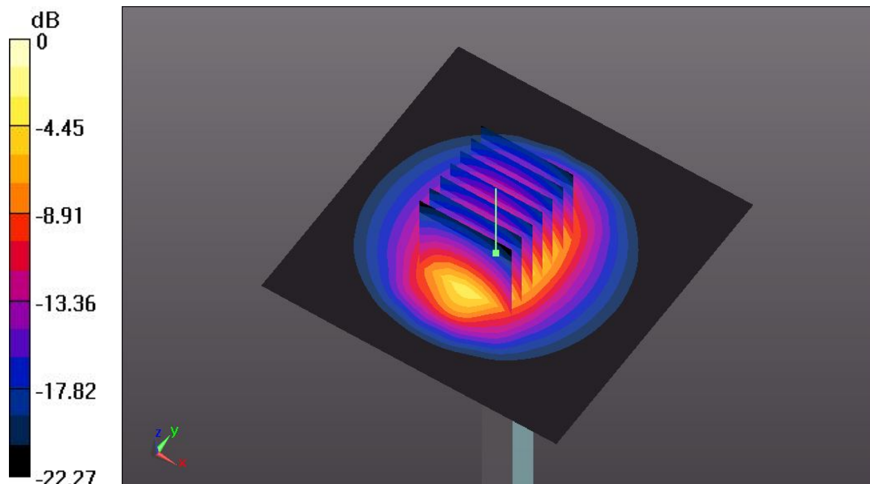
0 dB = 19.8 W/kg
