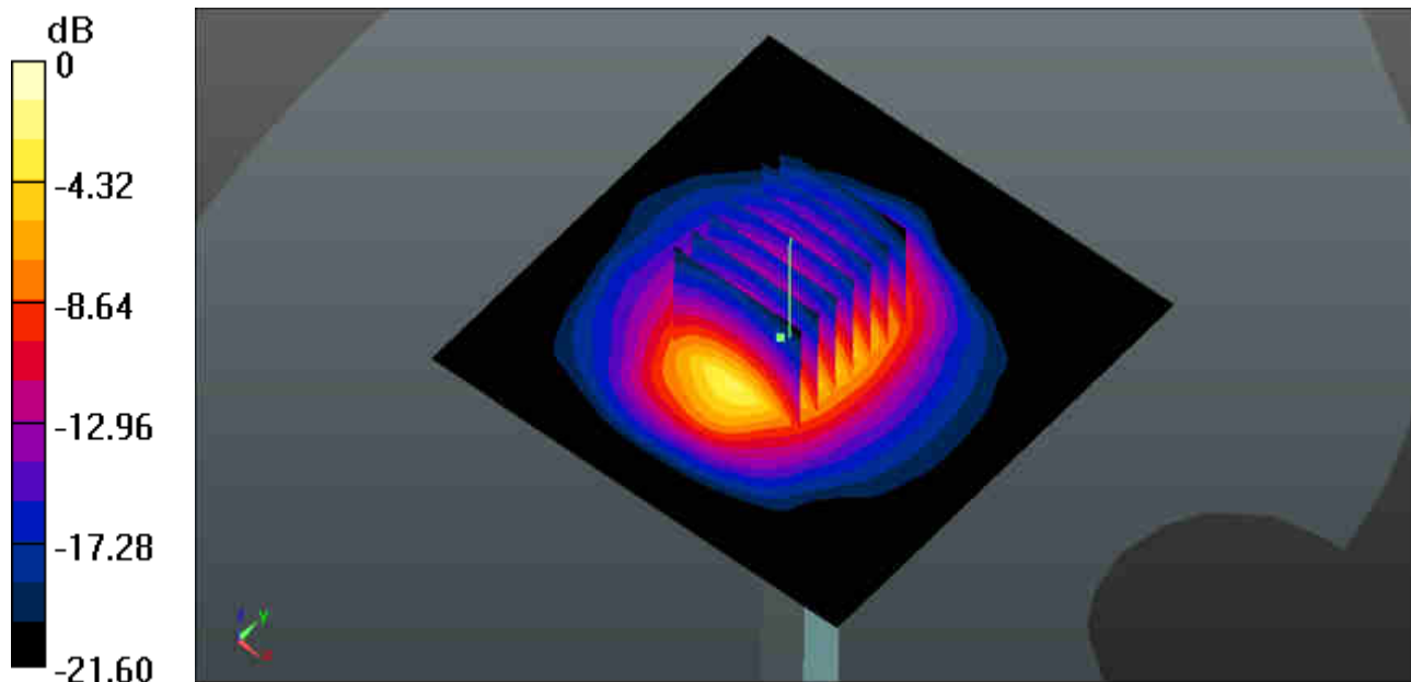
0 dB = 20.1 W/kg
