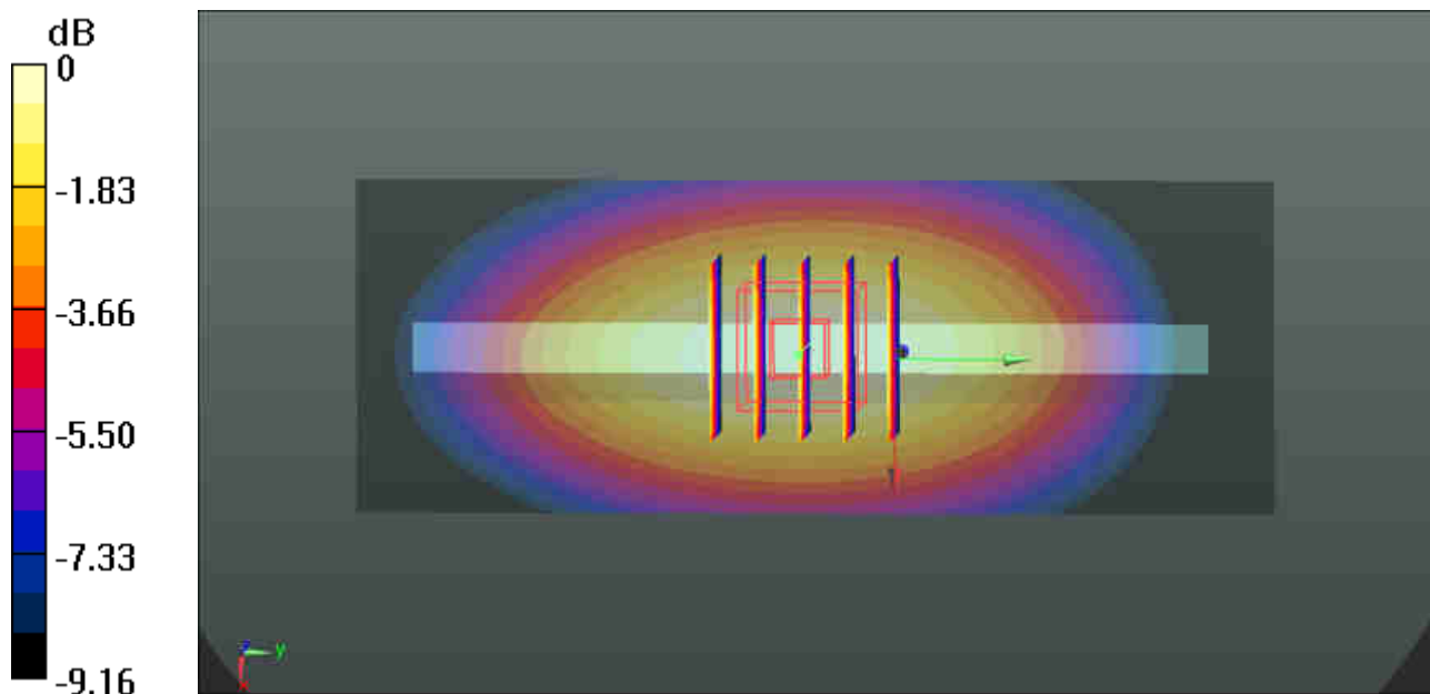
0 dB = 0.409 W/kg
