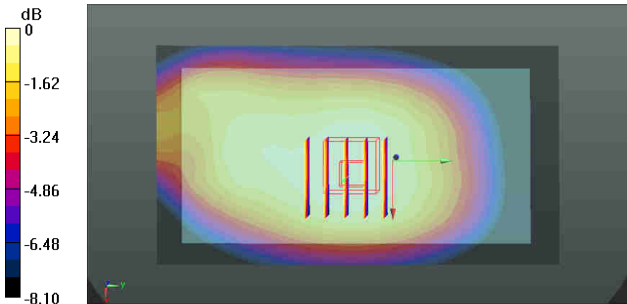
0 dB = 0.371 W/kg
